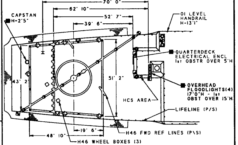
AVERAGE CLASS HELO DECK HEIGHT ABOVE WATERLINE: 15' 10" (MAIN DECK AFT)
