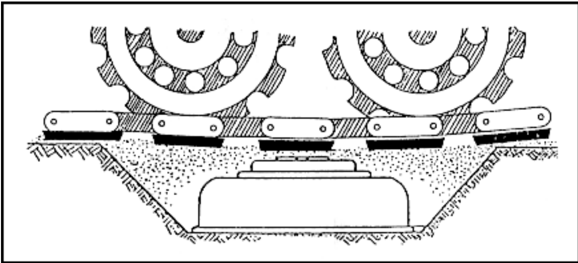
Figure 5-5. Buried mine with pressure plate
