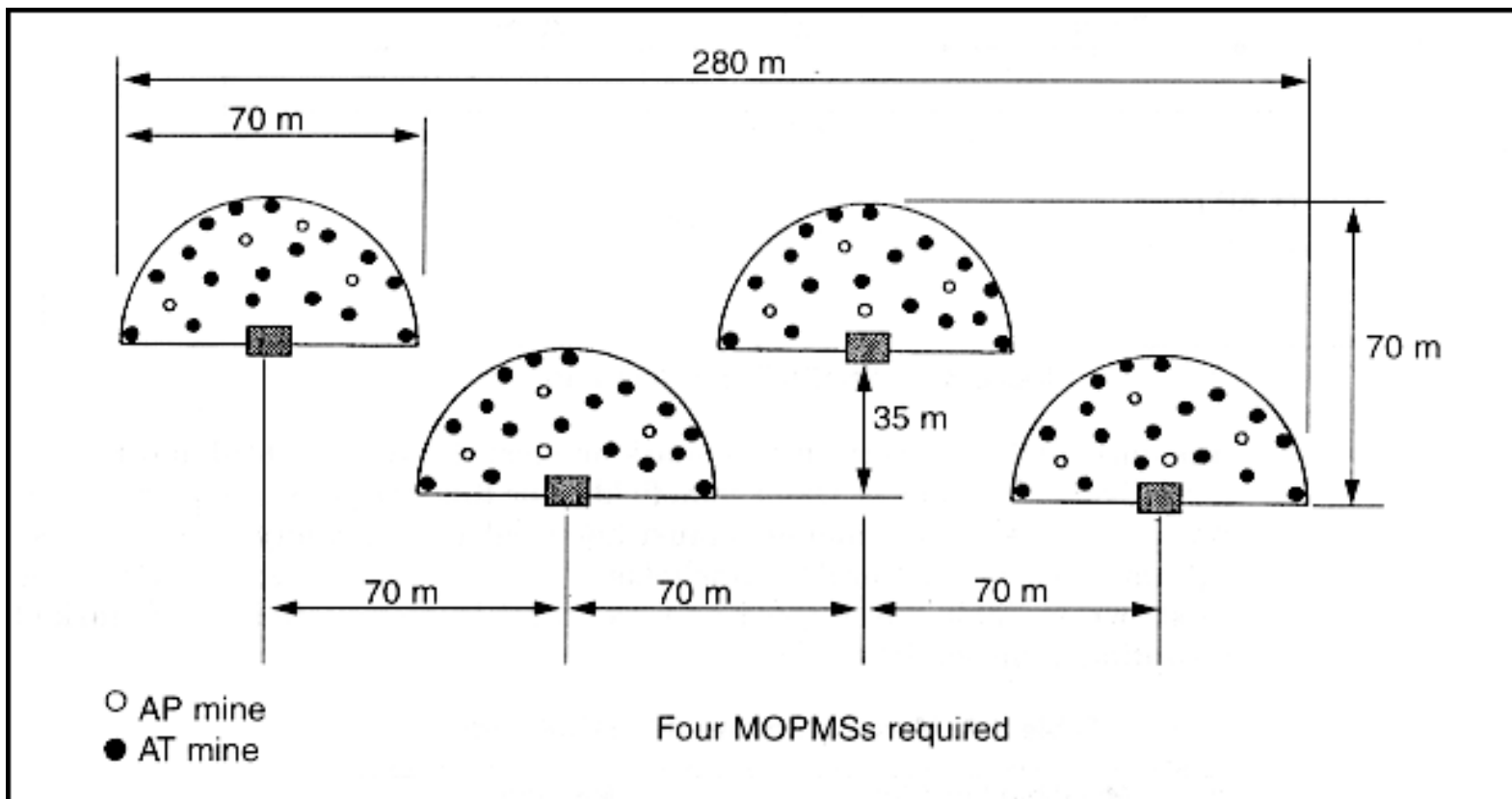
Figure 3-16. MOPMS in a disrupt minefield
