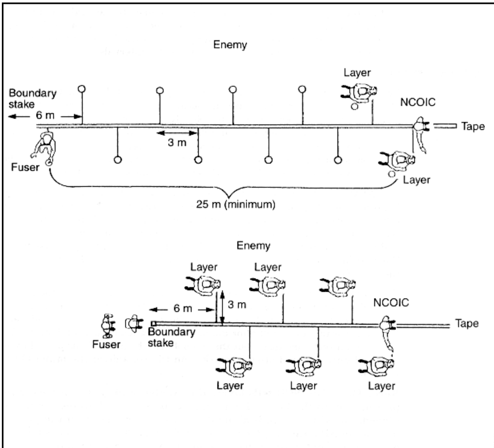
Figure 7-8. Laying and fusing mines
