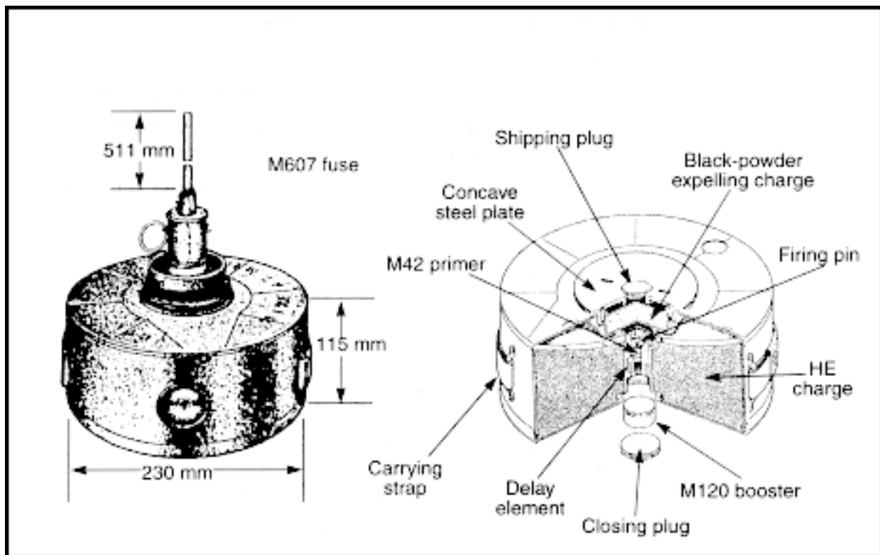
Figure A-29. M21 AT mine
