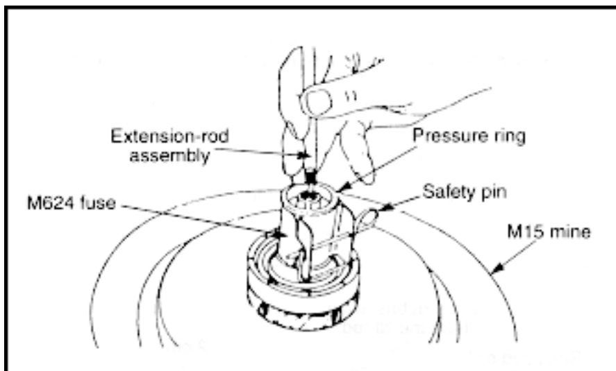
Figure A-18. Extension-rod assembly
