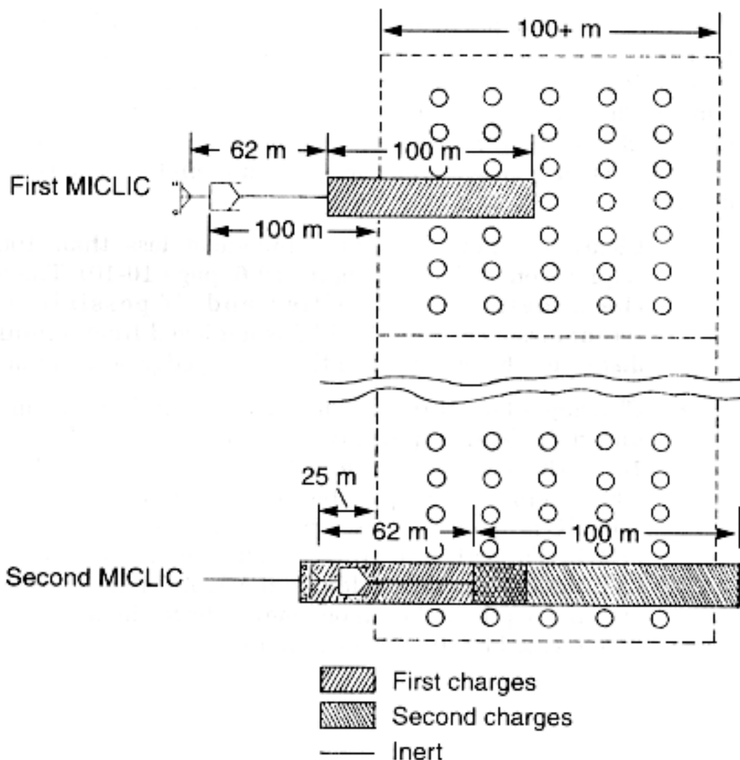
Figure 10-7. MICLIC employment in a minefield of uncertain depth or greater than 100 meters
