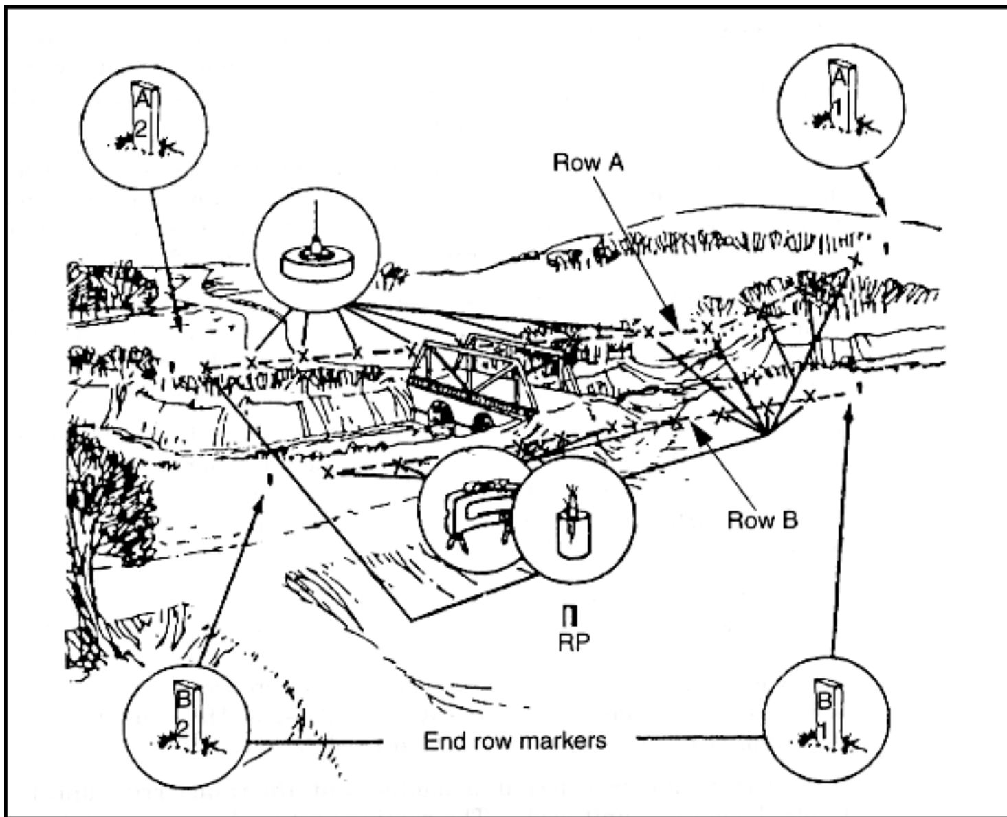
Figure 6-13. Site layout
