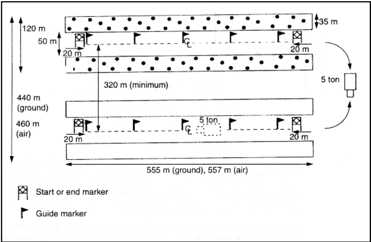
Figure 3-13. Volcano turn and block minefields
