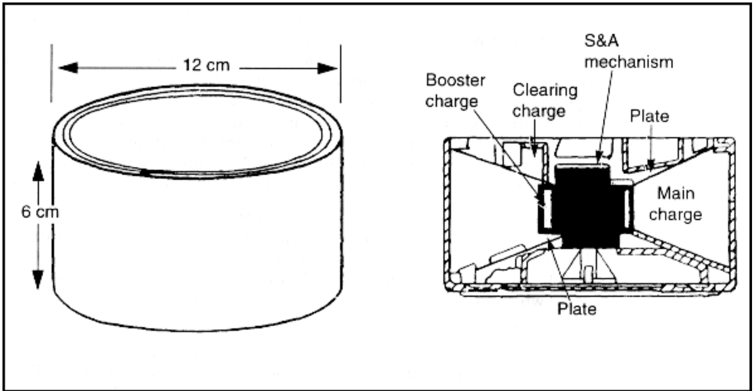
Figure 3-2. AT SCATMINE
