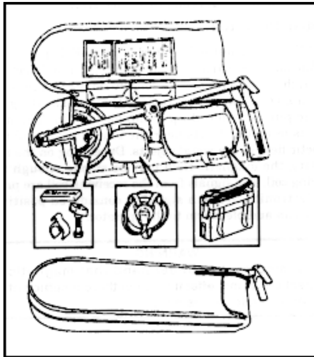
Figure F-2. AN/PSS-12 packed components
