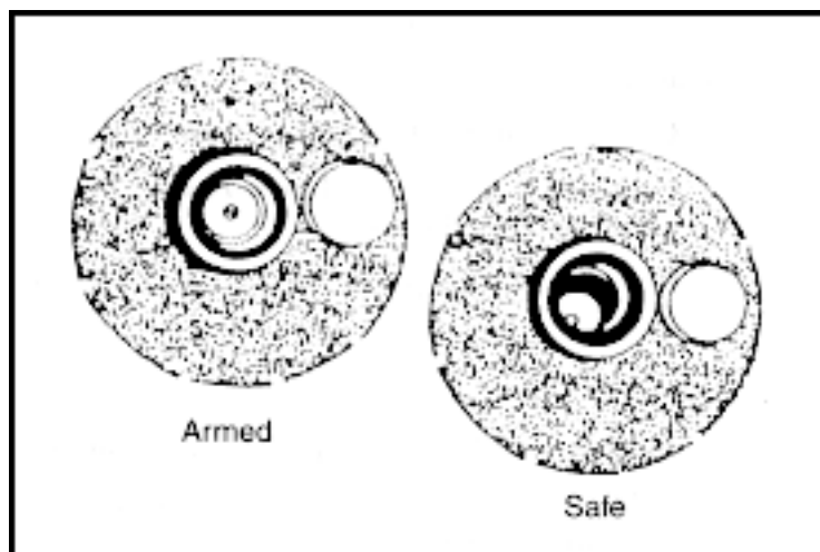
Figure A-28. Firing pin
