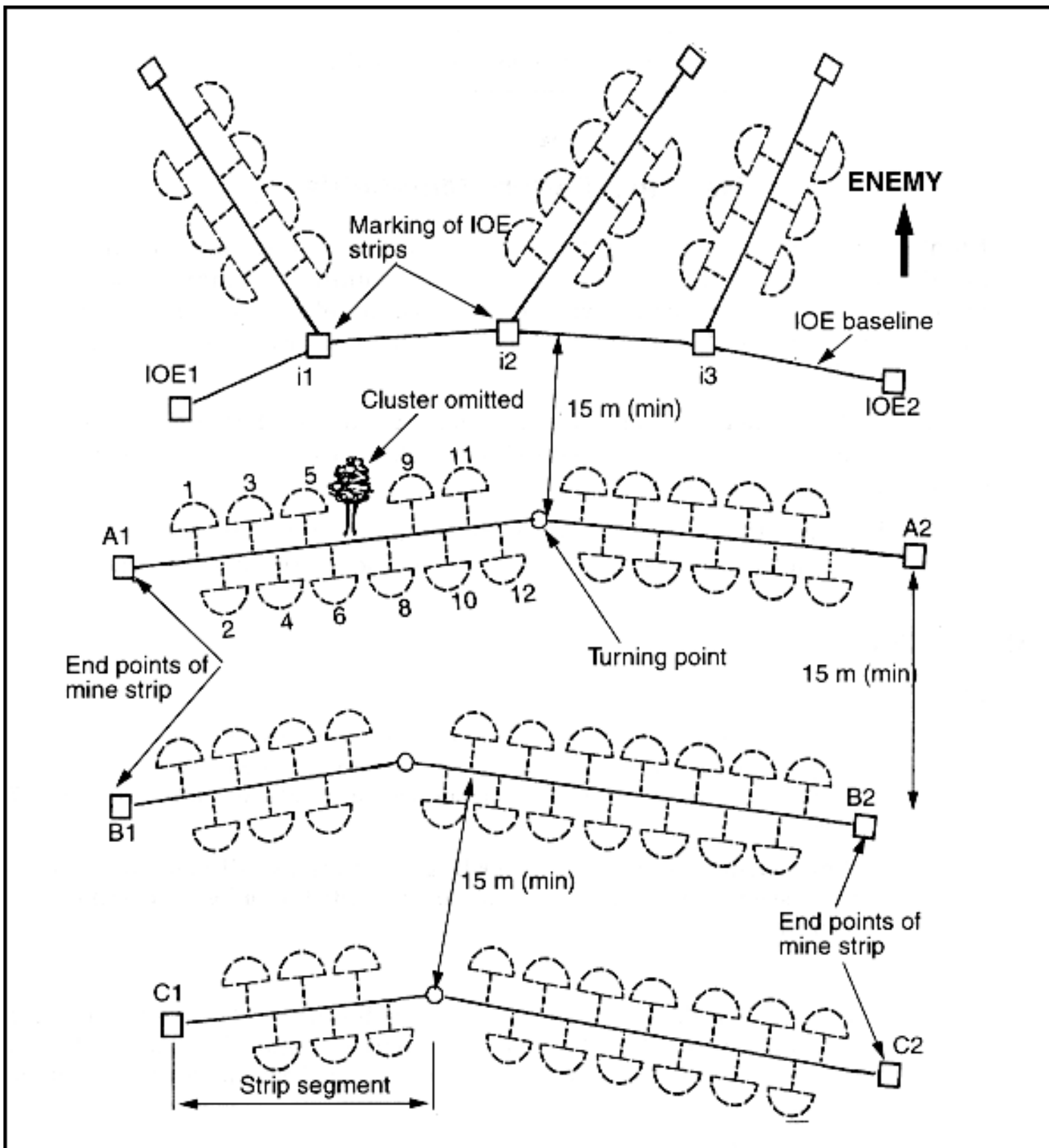
Figure 7-1. Minefield layout
