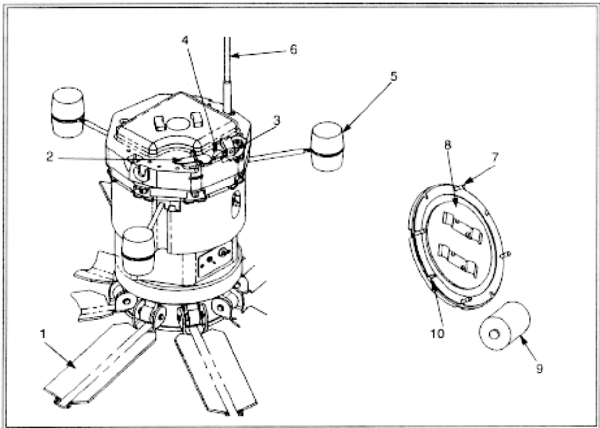
Figure B-3. Hornet components
