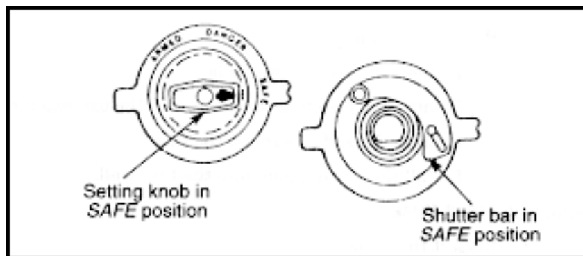
Figure A-22. SAFE position
