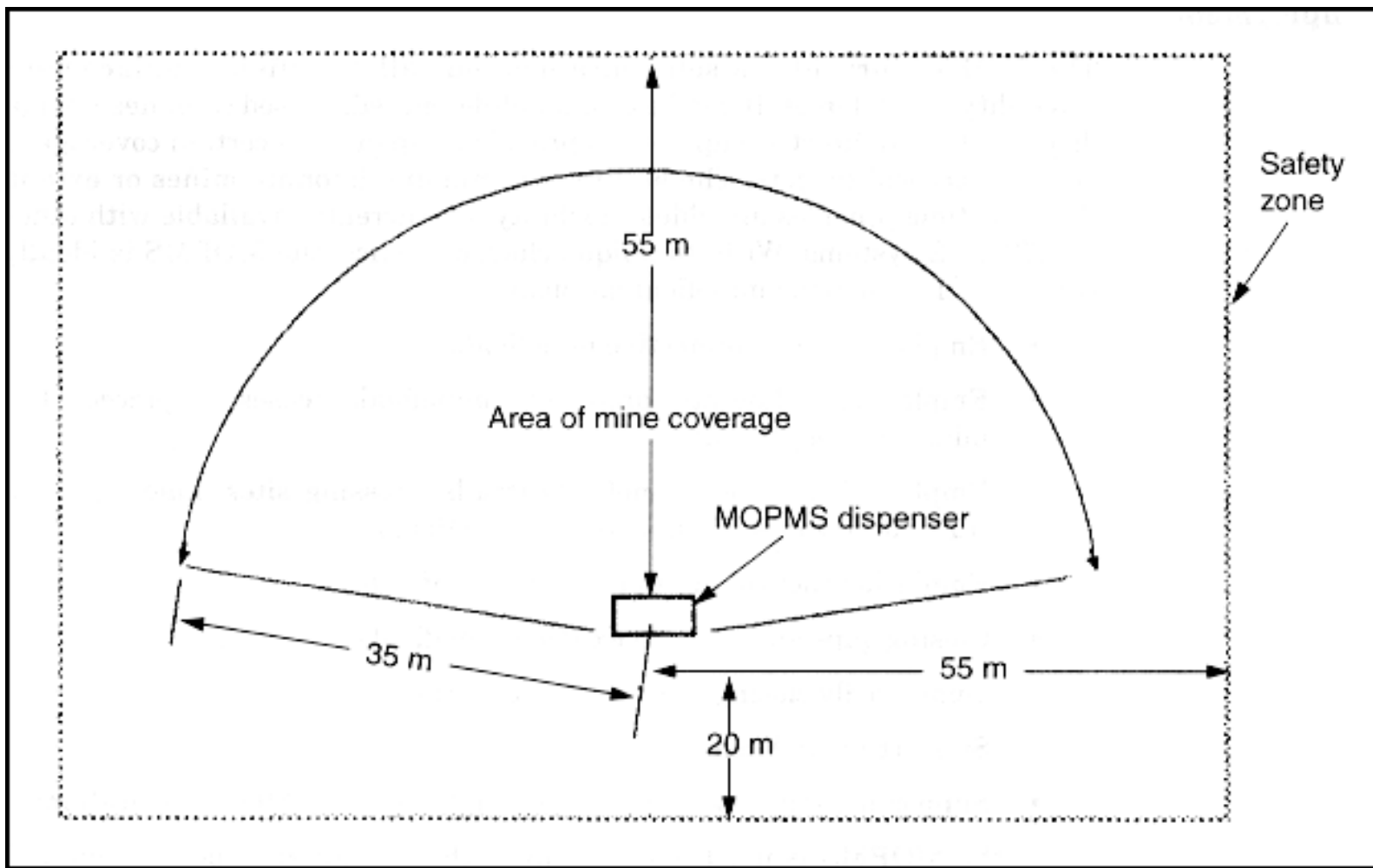
Figure 3-15. MOPMS emplacement and safety zone
