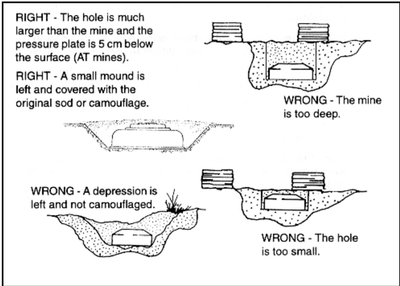
Figure 5-7. Buried and concealed mines
