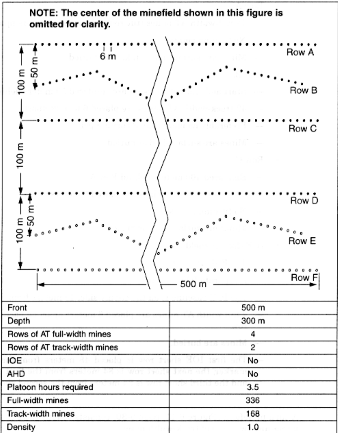
Figure 6-11. Standardized turn row minefield
