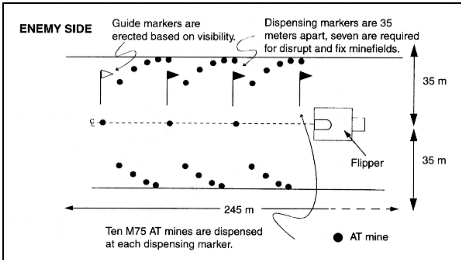
Figure 3-8. Flipper disrupt and fix minefields
