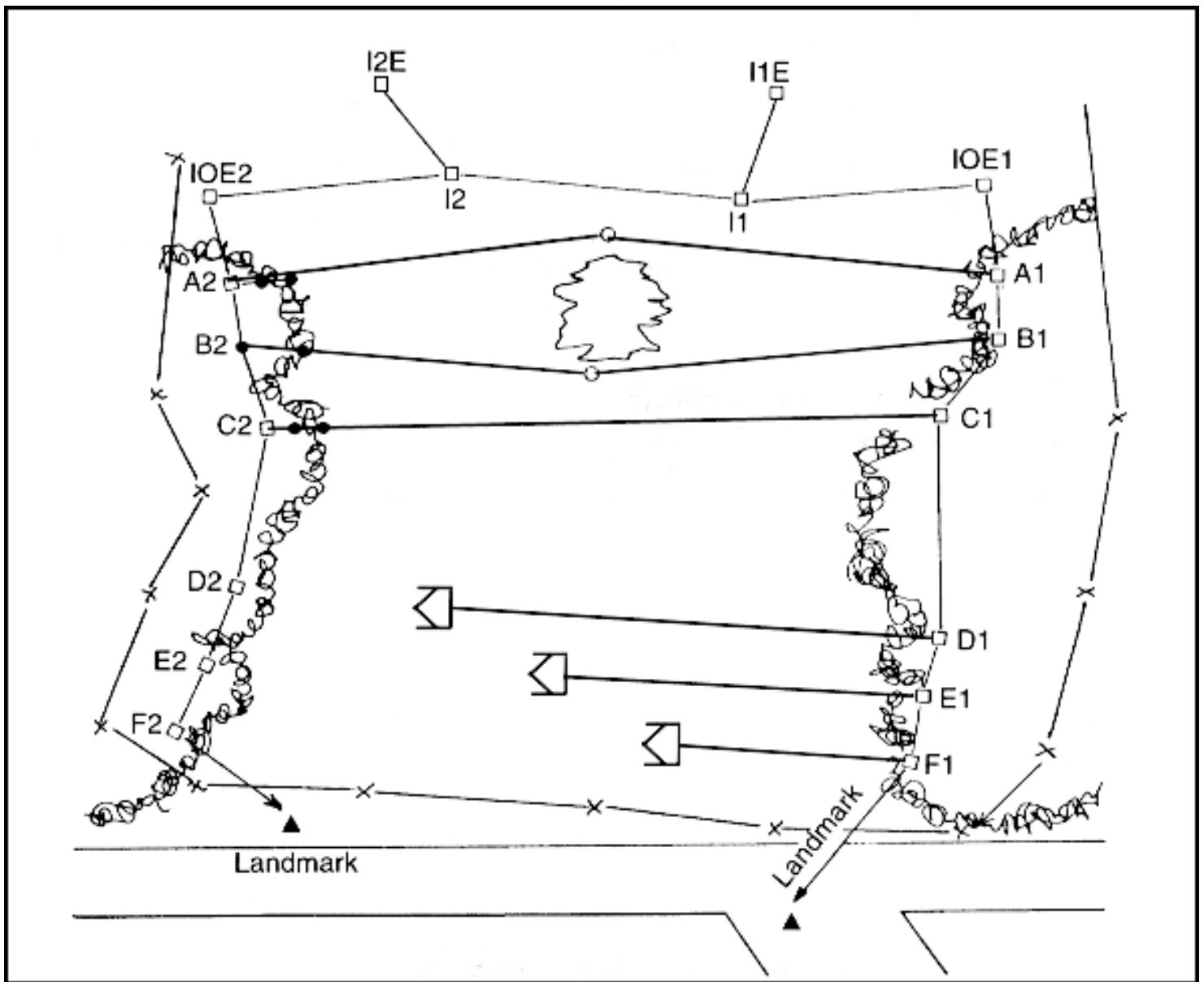
Figure 6-4b. Laying a minefield (continued)
