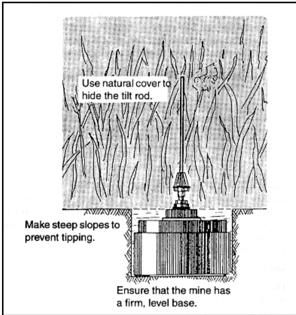
Figure 5-6. Buried mine with tilt rod
