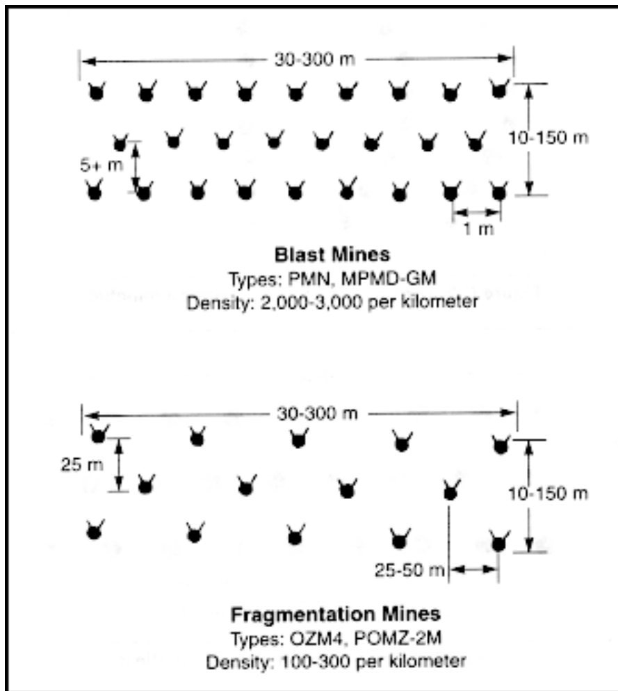
Figure C-5. Threat-style AP minefield
