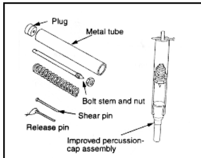
Figure 13-8. Improved nonelectrical FDs (spring-operated)
