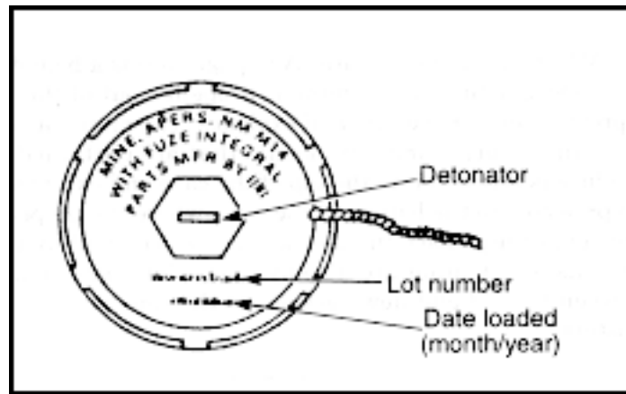
Figure A-5. Bottom view of M14 mine
