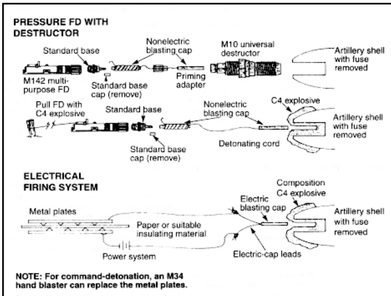
Figure 13-15. HE, artillery-shell AT device
