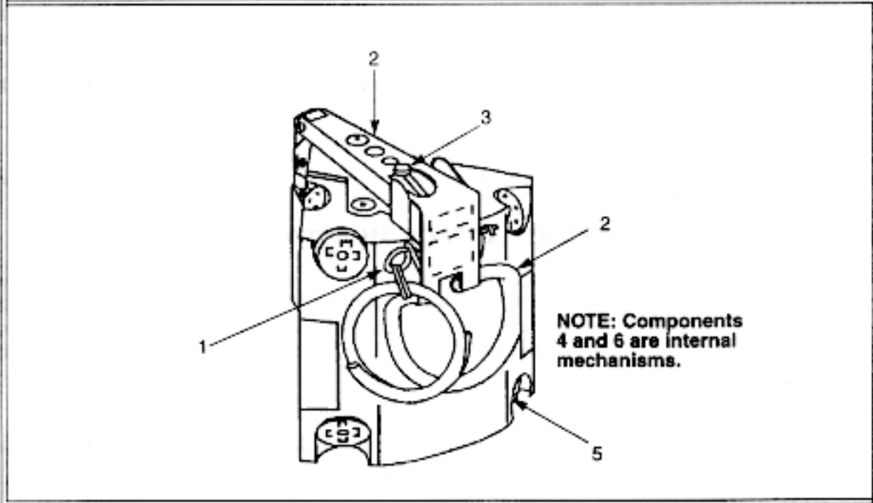
Figure B-1. PDM components
