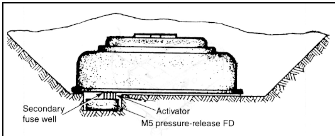
Figure 1-4. AHD incorporating a release mechanism
