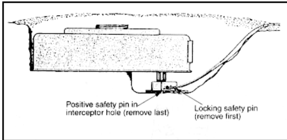
Figure A-35. Arming the M15
