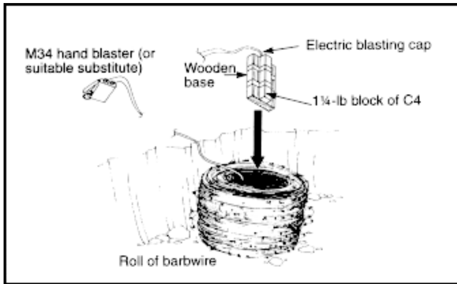
Figure 13-19. Barbwire AP device
