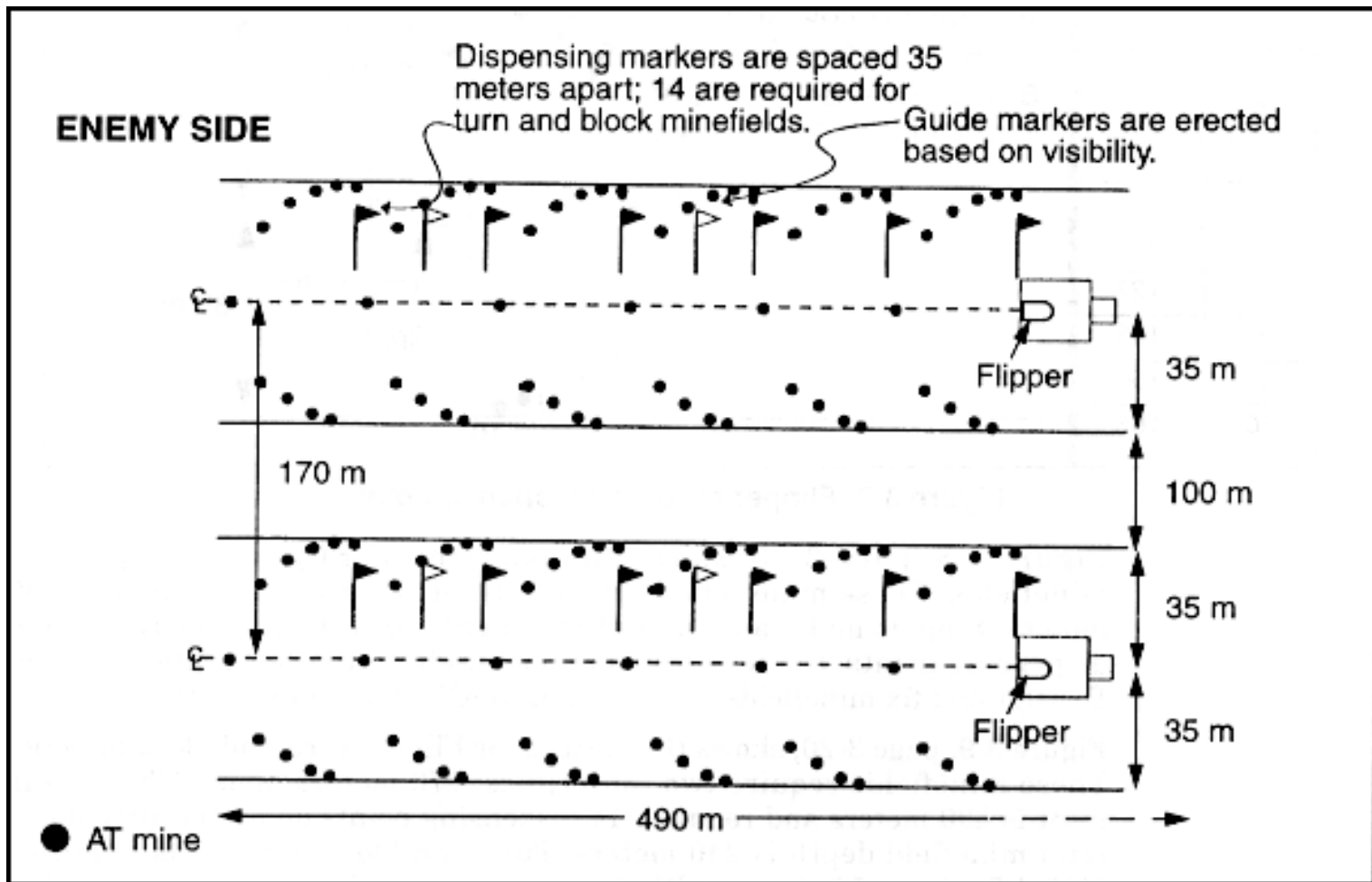
Figure 3-9. Flipper turn and block minefields
