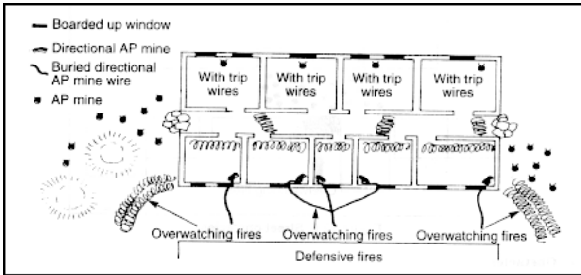
Figure 12-8. Building obstacles
