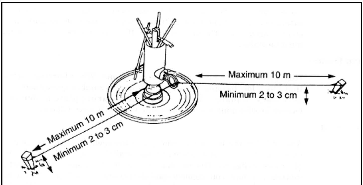
Figure 5-4. Trip-wire-activated AP mine
