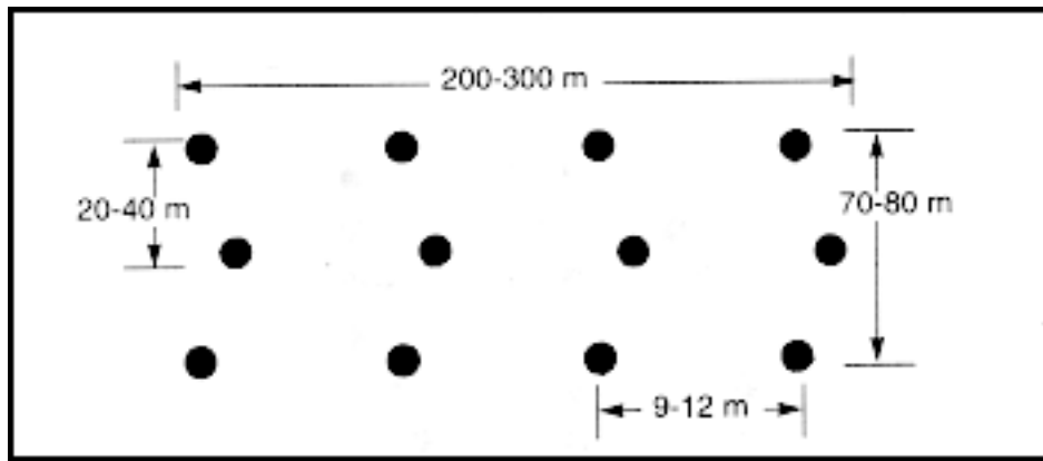
Figure C-4. Threat-style antihull minefield
