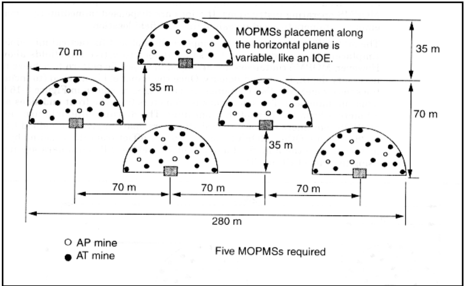
Figure 3-17. MOPMS in a fix minefield
