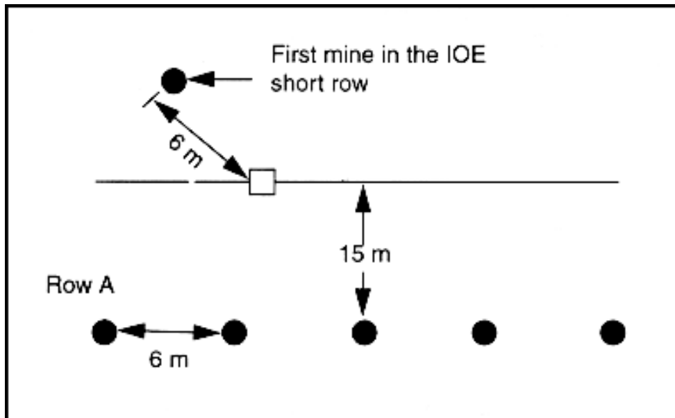
Figure 6-5. Laying an IOE short row
