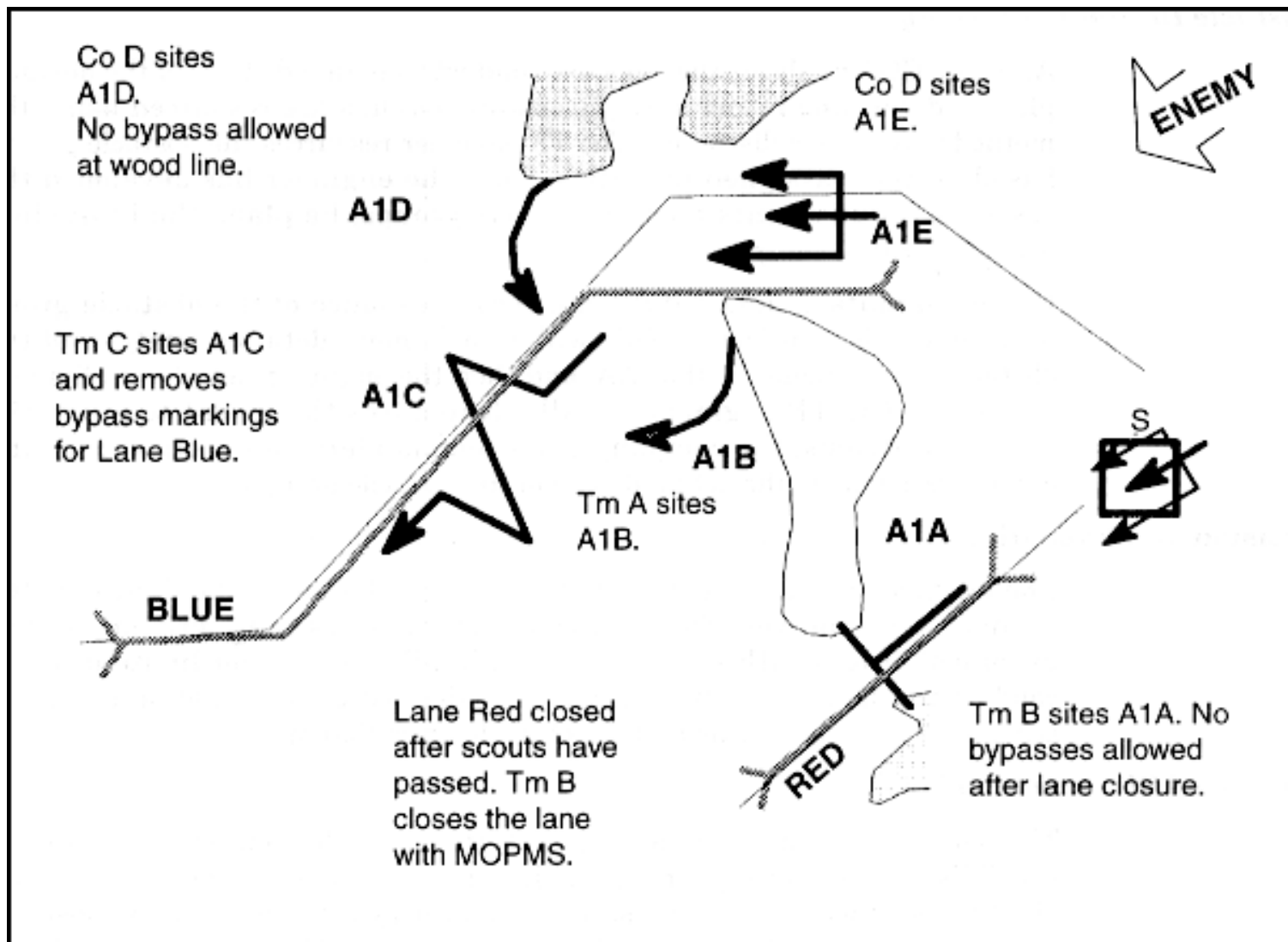
Figure 2-16. Scheme-of-obstacle overlay
