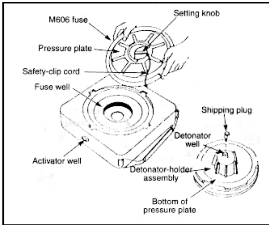
Figure A-27. Removal of the pressure plate
