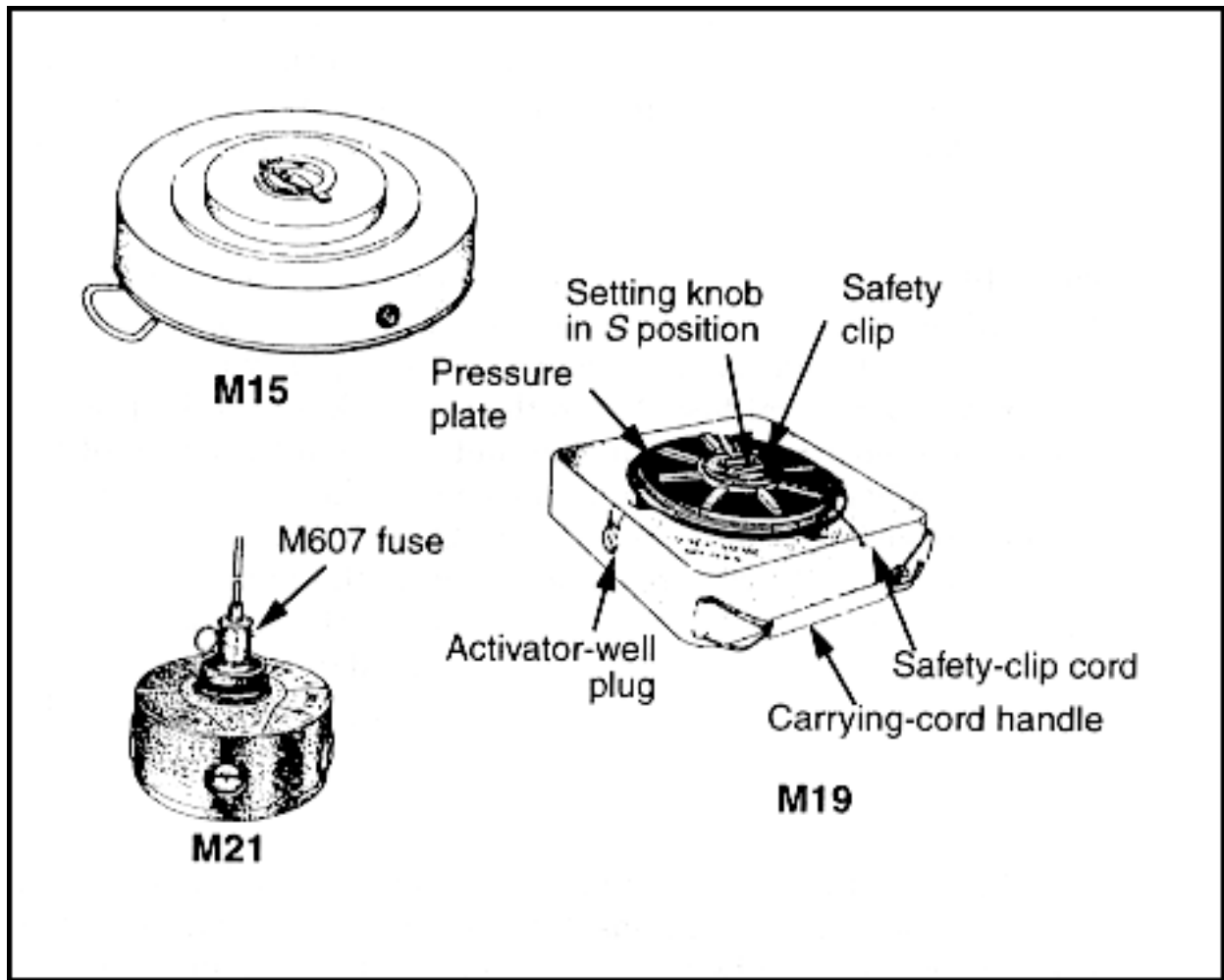
Figure 5-1. AT mines
