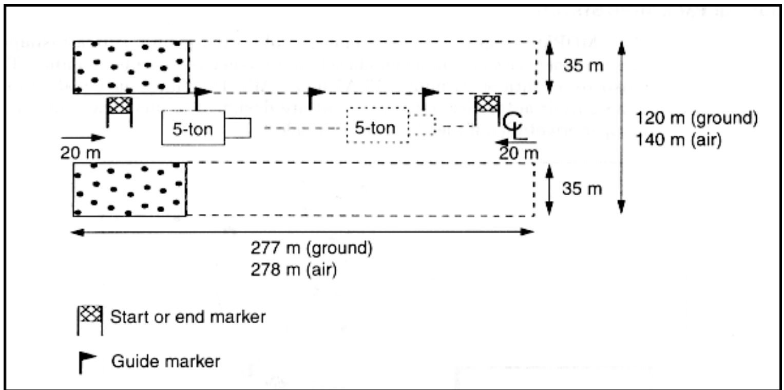
Figure 3-12. Volcano disrupt and fix minefields
