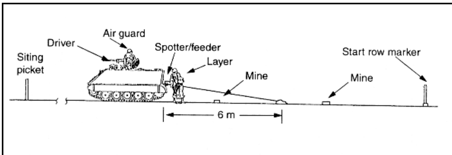
Figure 6-8. Measuring distances between mines with sandbags
