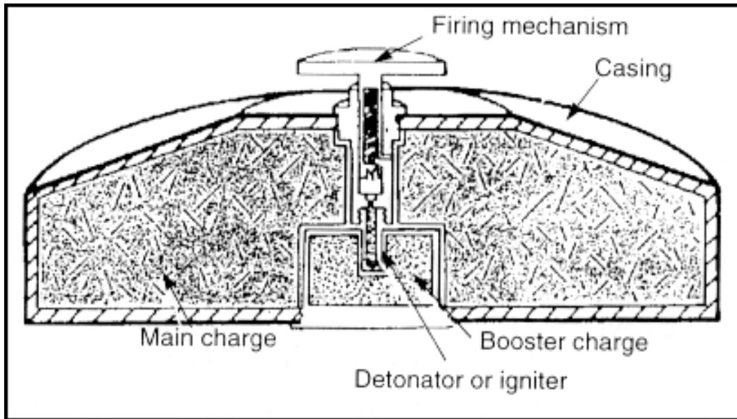
Figure 1-1. Mine components
