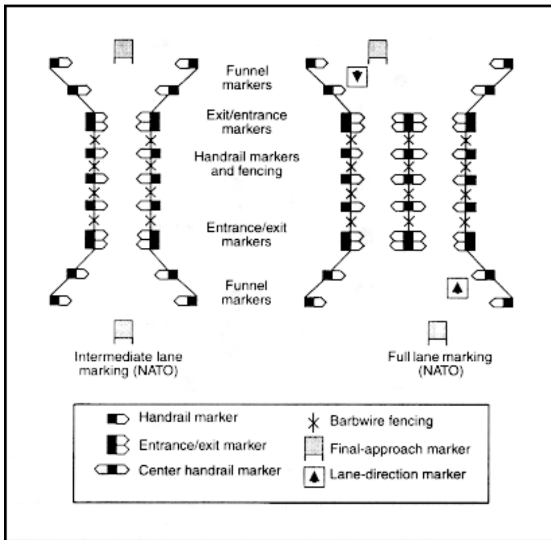
Figure 10-27. NATO lane-marking conversion
