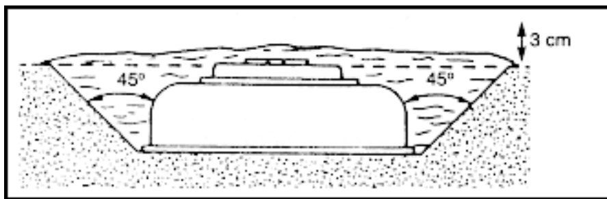
Figure A-25. M15 mine in the hole
