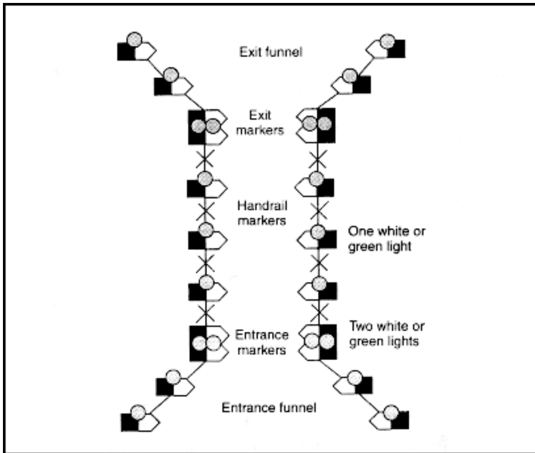
Figure 10-28. NATO standard marking for limited visibility
