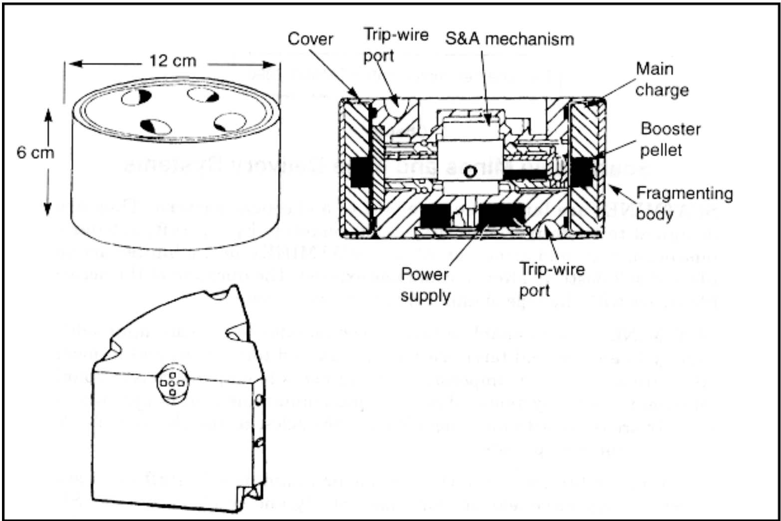
Figure 3-1. AP SCATMINES
