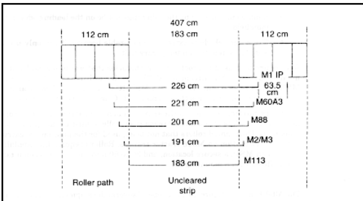
Figure 10-16. Mine-roller width compared to track-vehicle widths
