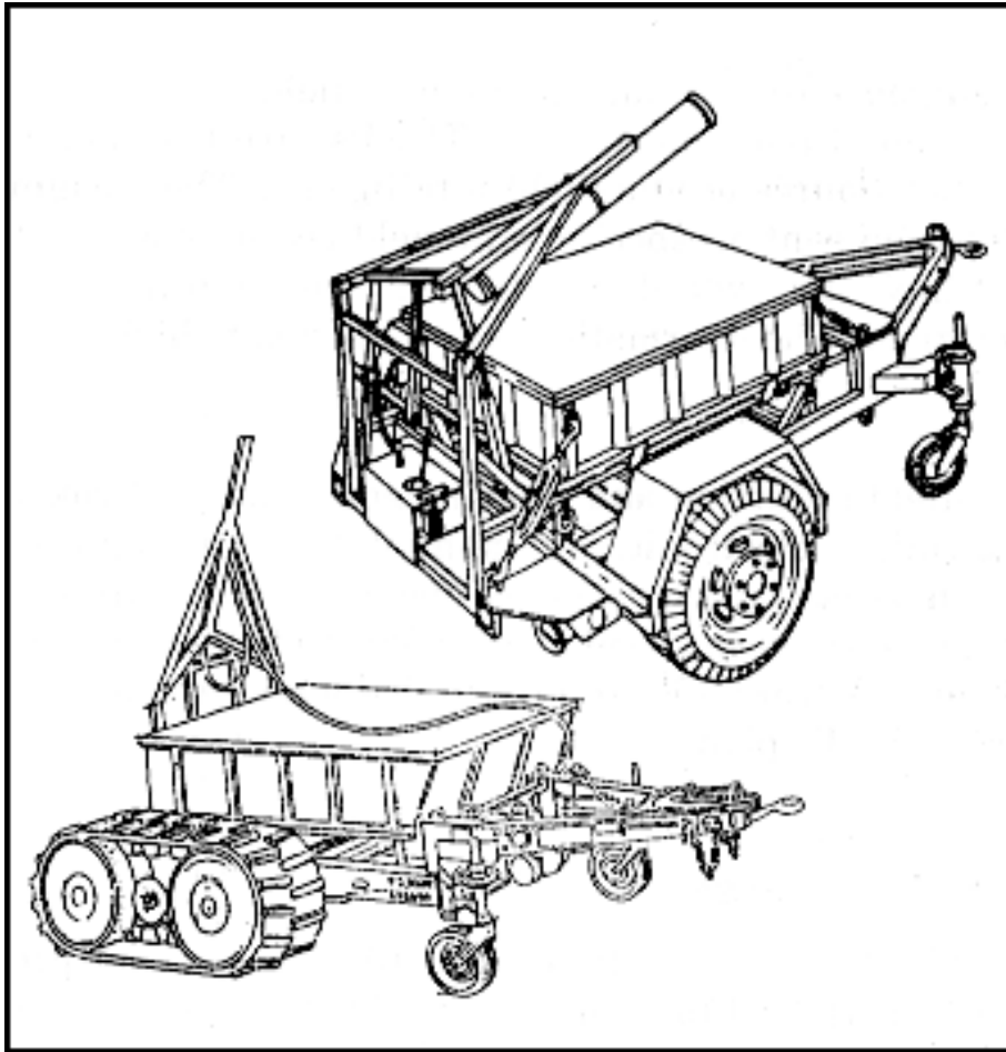
Figure 10-4. MICLIC
