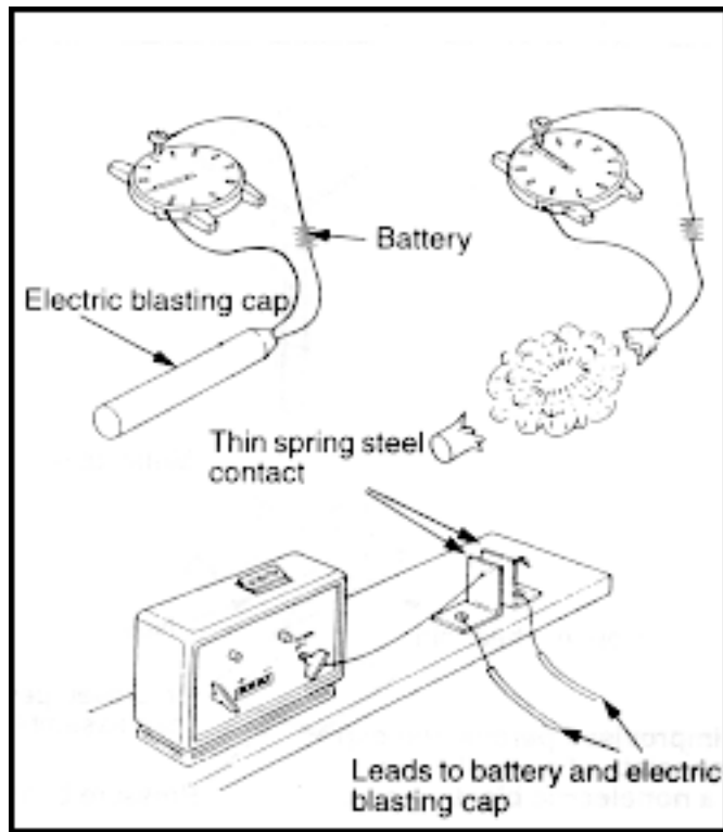
Figure 13-9. Improvised, electric delay devices
