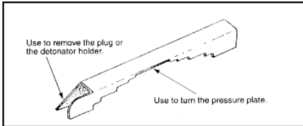
Figure A-2. M22 wrench
