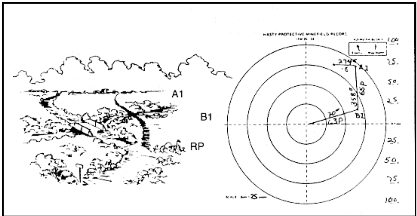
Figure 8-5. Hasty protective row minefield/munition field record
