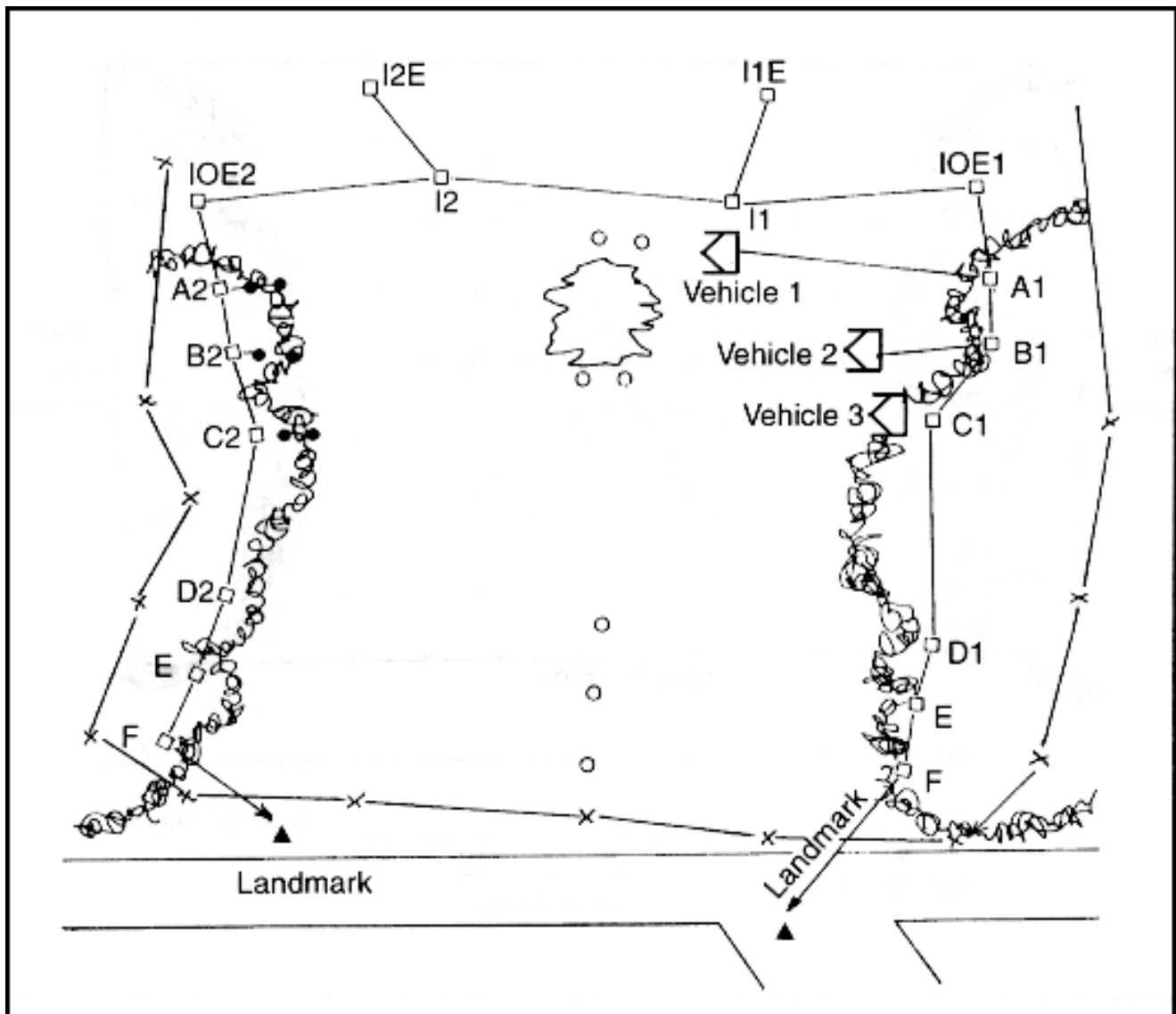
Figure 6-4a. Laying a minefield
