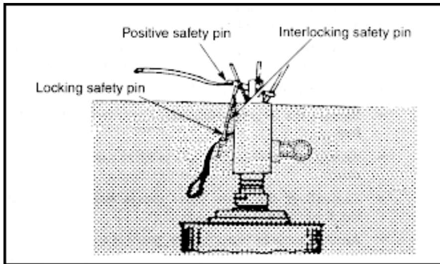
Figure A-9. Safety pins
