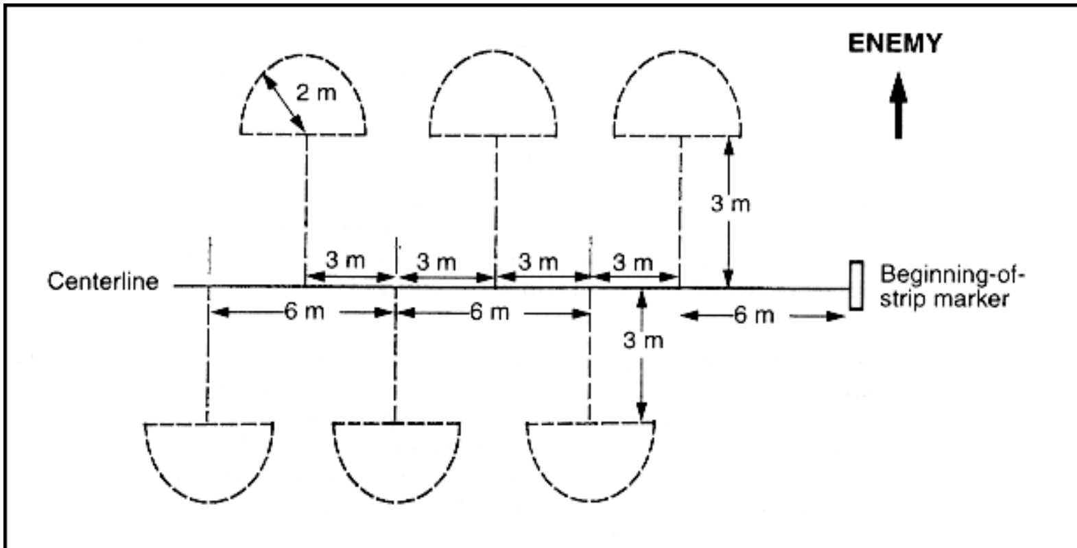
Figure 7-3. Arrangement of clusters in a mine strip
