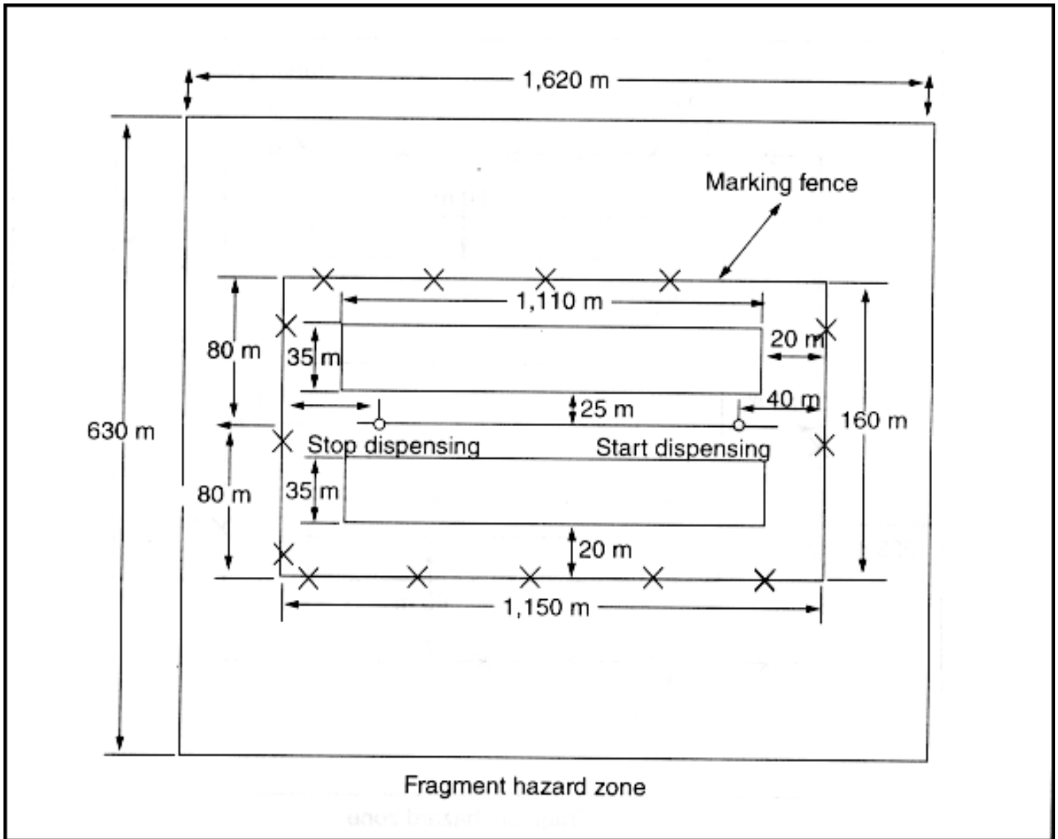
Figure 3-19. Ground Volcano minefield
