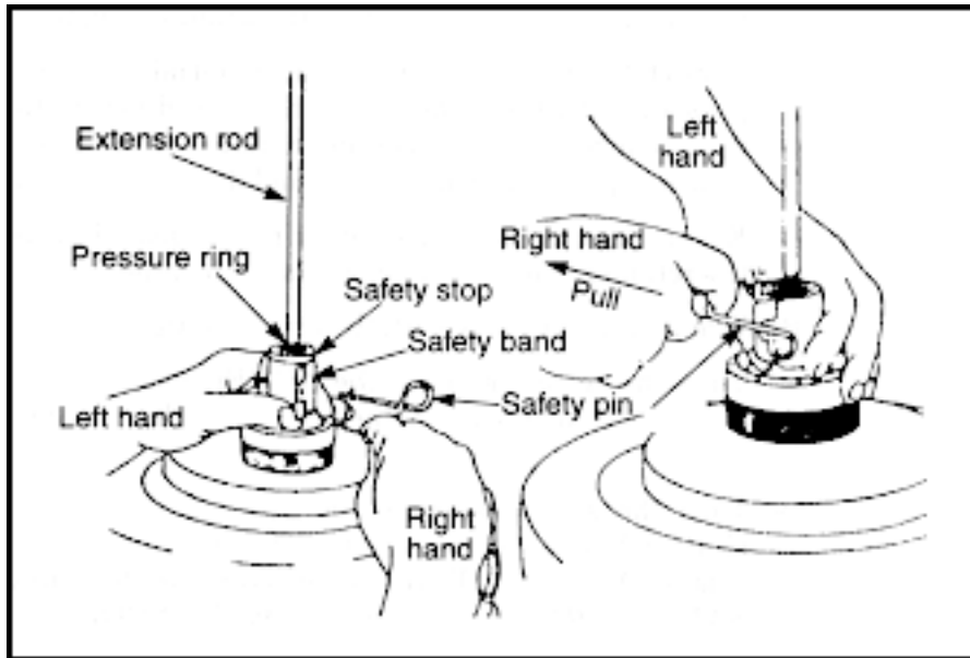
Figure A-20. Removal of safety pin
