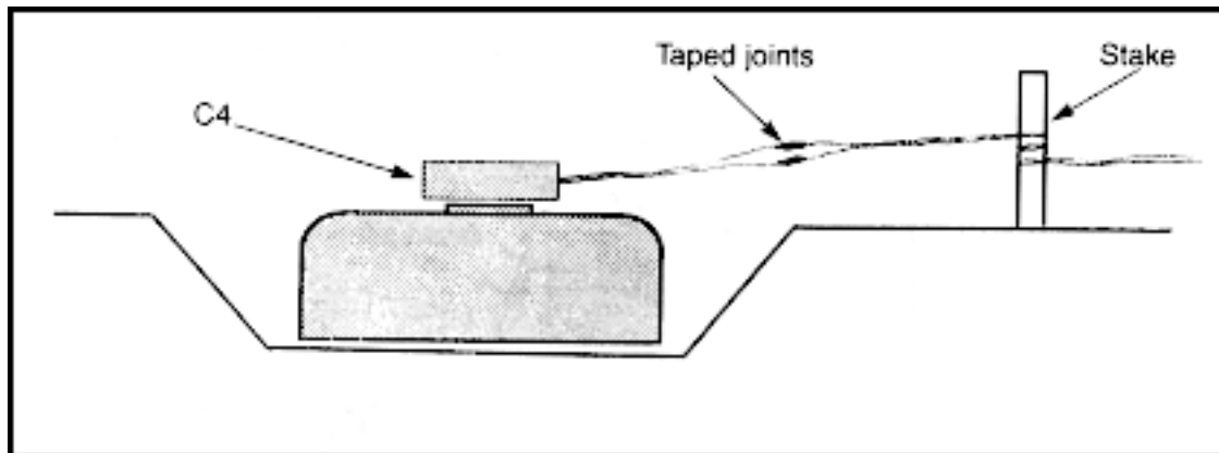
Figure E-3. M15 and M19 AT mines
