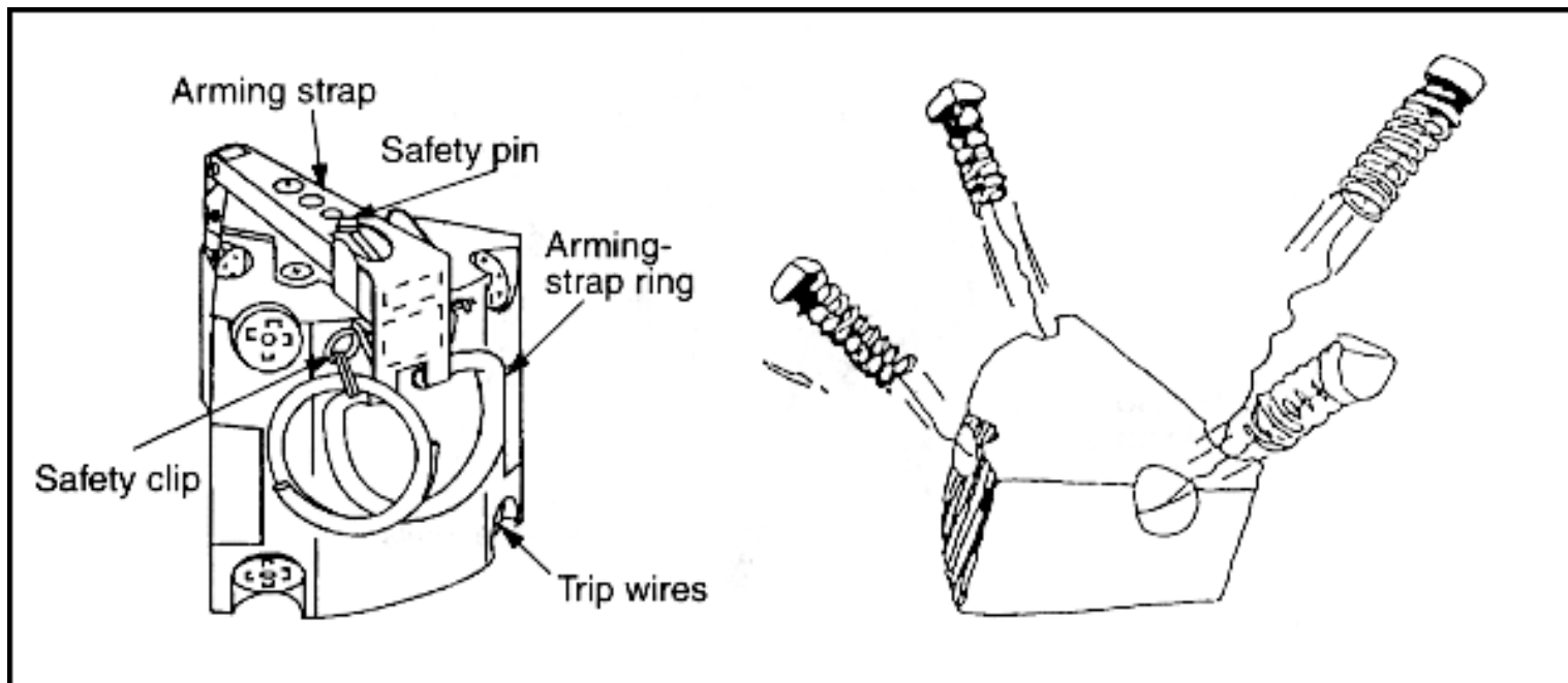
Figure 4-1. M86 PDM
