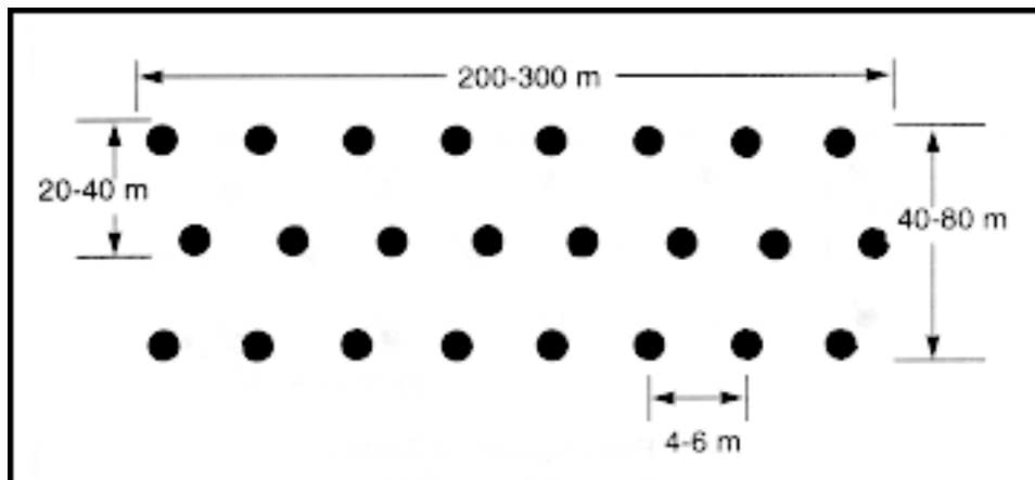
Figure C-3. Threat-style antitrack minefield
