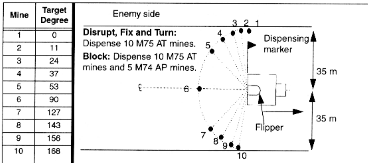
Figure 3-7. Flipper stop-and-dispense point
