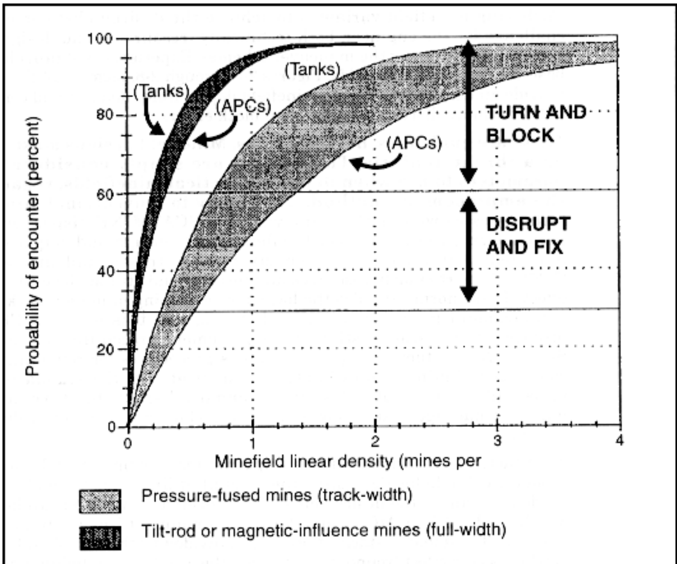
Figure 2-4. Vehicle mine encounter probability versus minefield density
