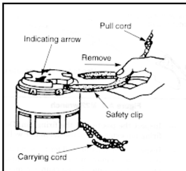
Figure A-4. Removal of safety clip
