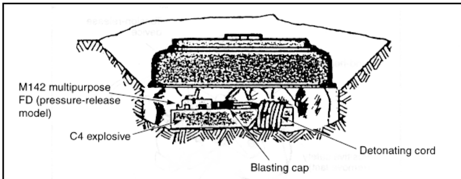
Figure 1-5. AHD not attached to the mine
