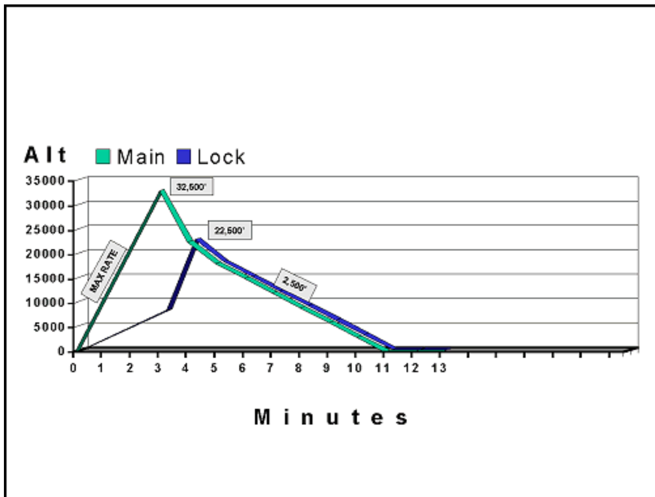
Figure A-5. Military Rapid Decompression Profile
