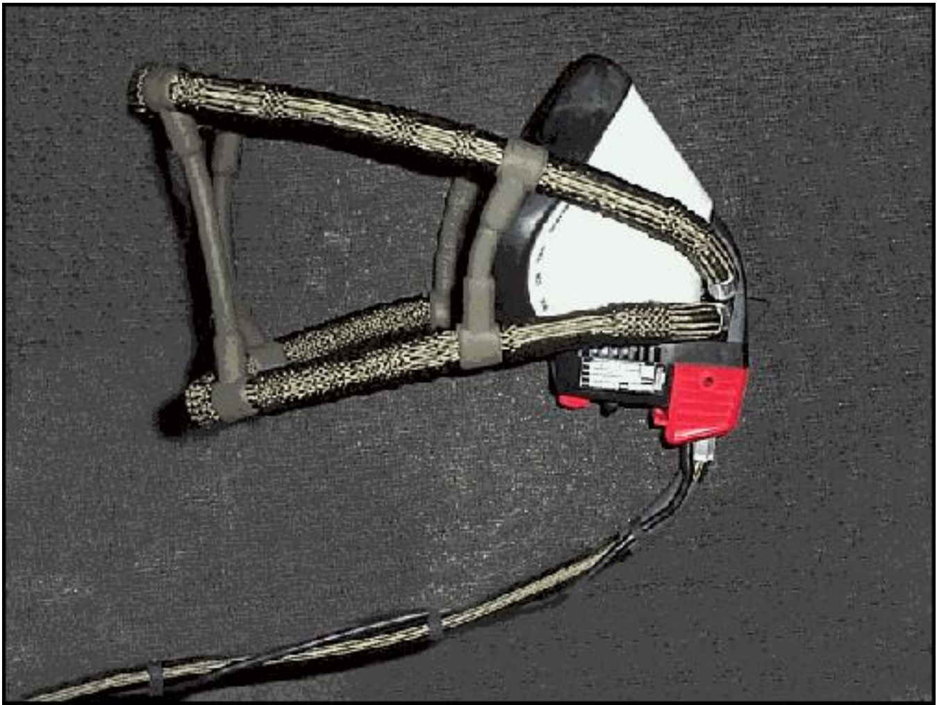
Figure 10-2. Quick-Donning Mask-Regulator
