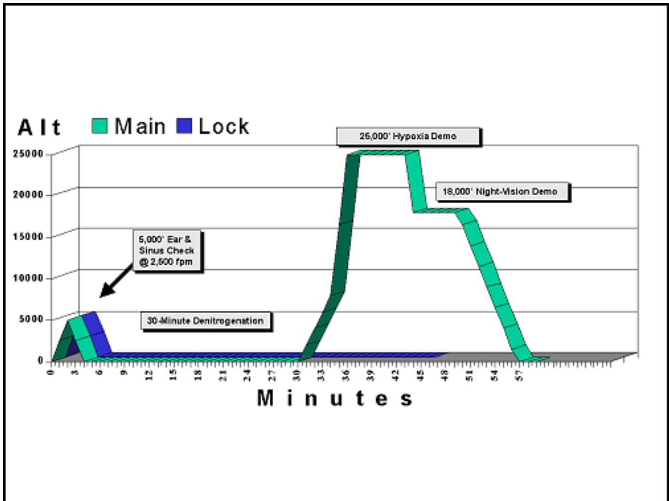
Figure A-3. Type IV, 25,000-Foot, USA Profile
