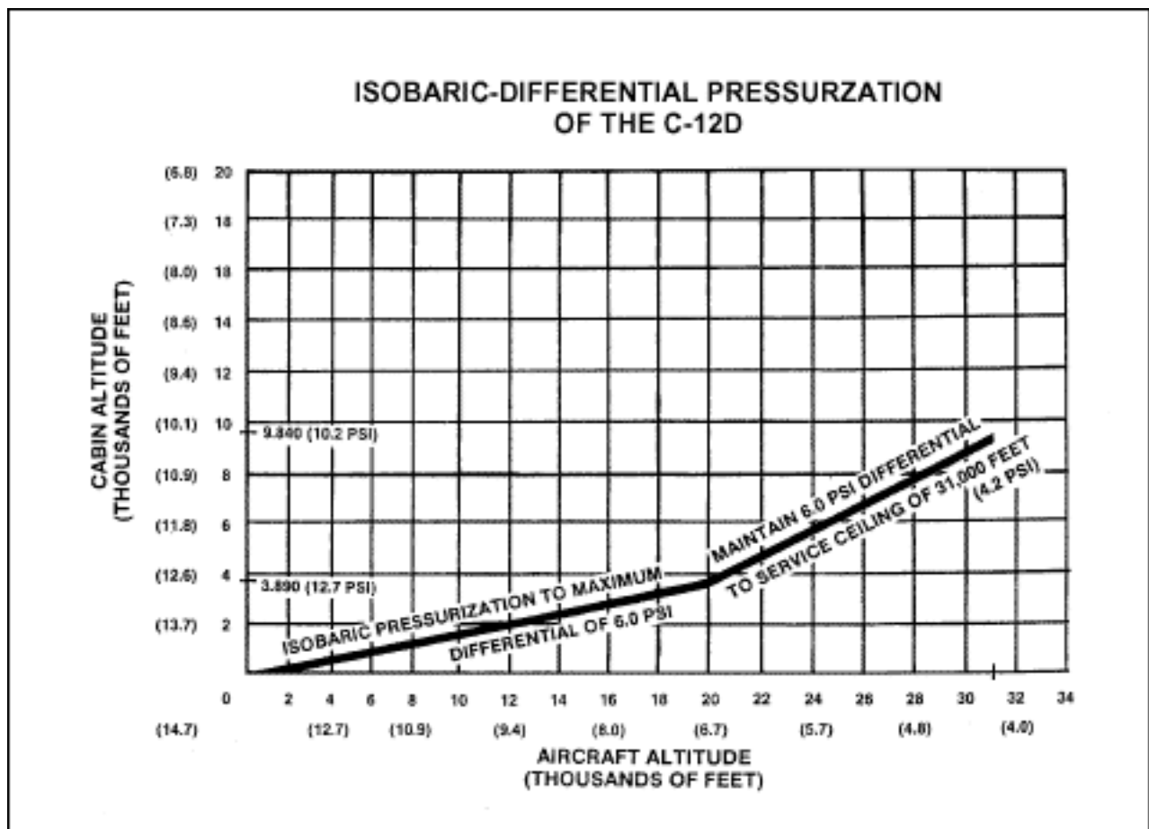
Figure 10-5. C-12D Cabin Pressurization Changes With Altitude Changes
