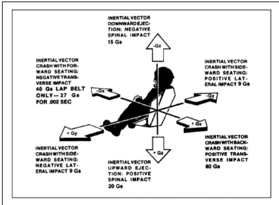
Figure 4-9. Human-Tolerance Limits to Whole-Body Impact (Duration 0.1 Second)
