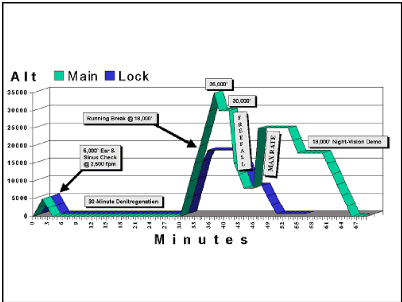
Figure A-4. Type V, 35,000-Foot, USA/USAF HAP
