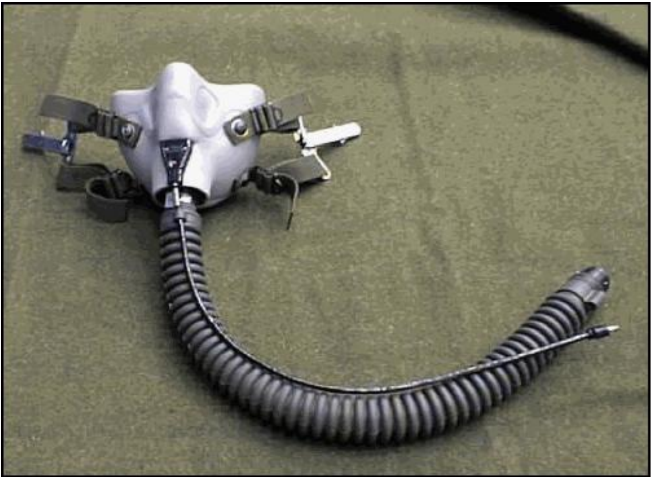
Figure 10-4. MBU-12/P Oxygen Mask
