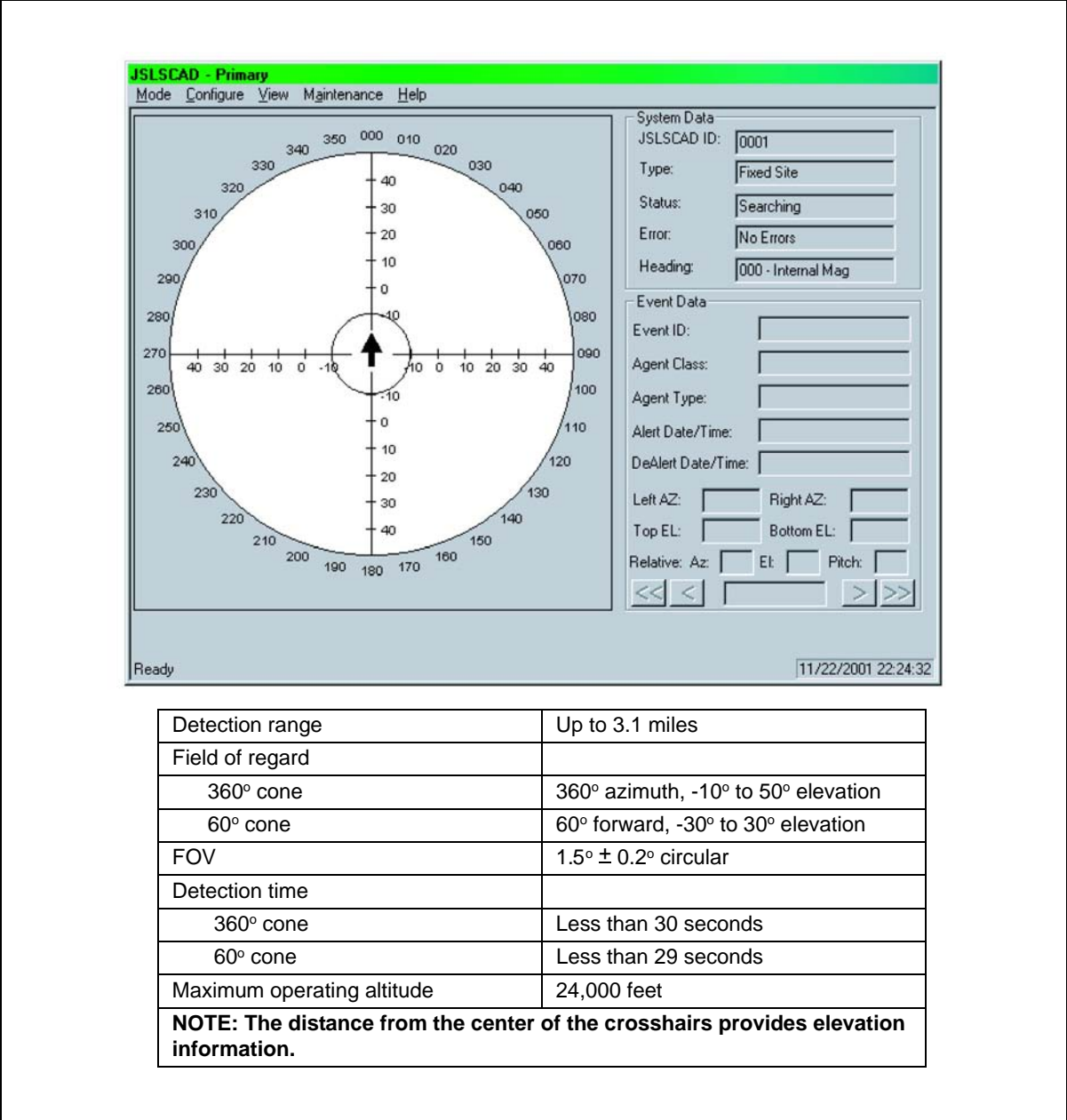
Figure M-1. Advanced Standoff Chemical Detector Performance Parameters
