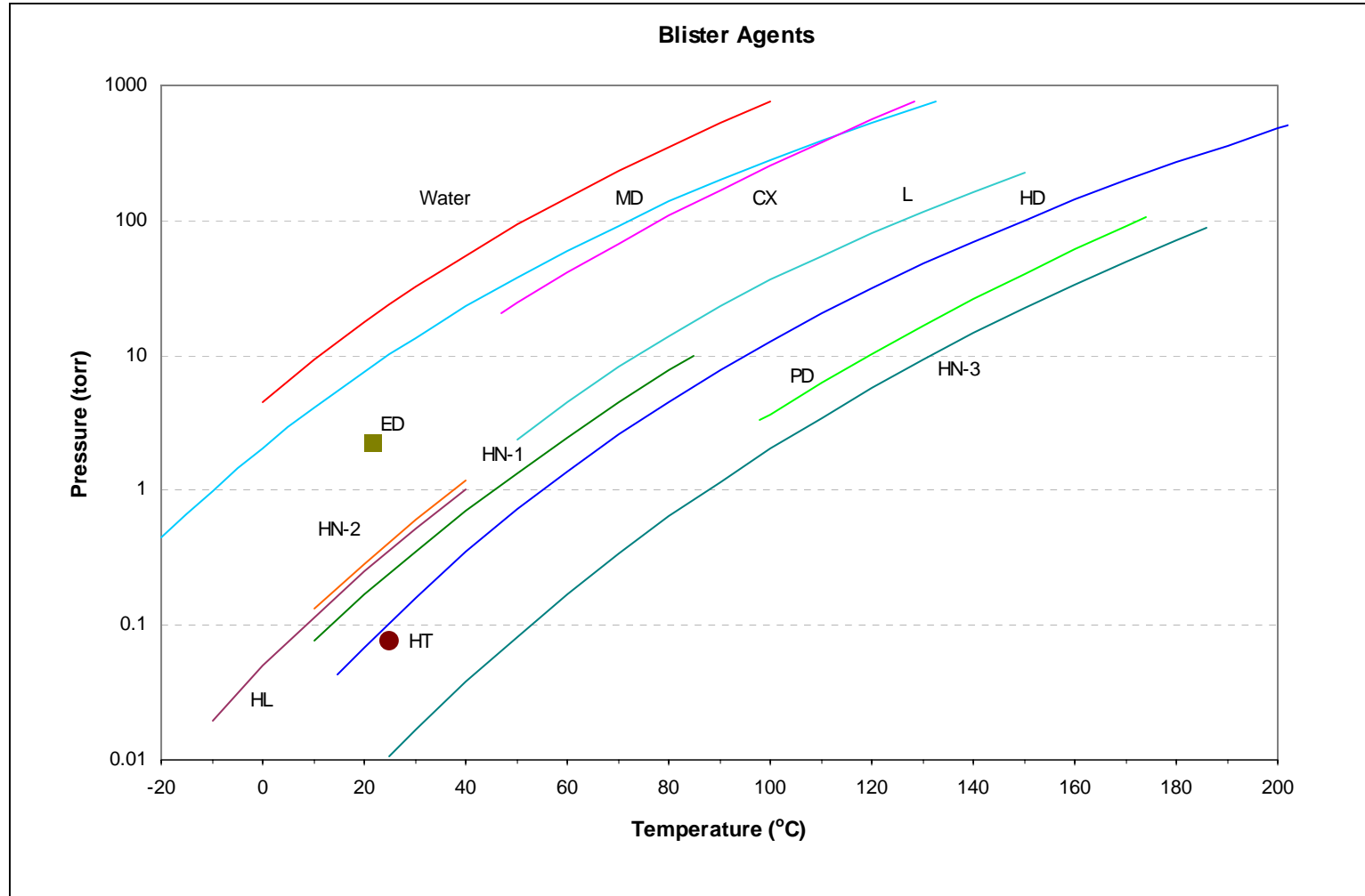
Figure G-4. Vapor Pressure of Blister Agents 1
