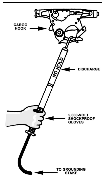
Figure 5-19. Grounding technique.
