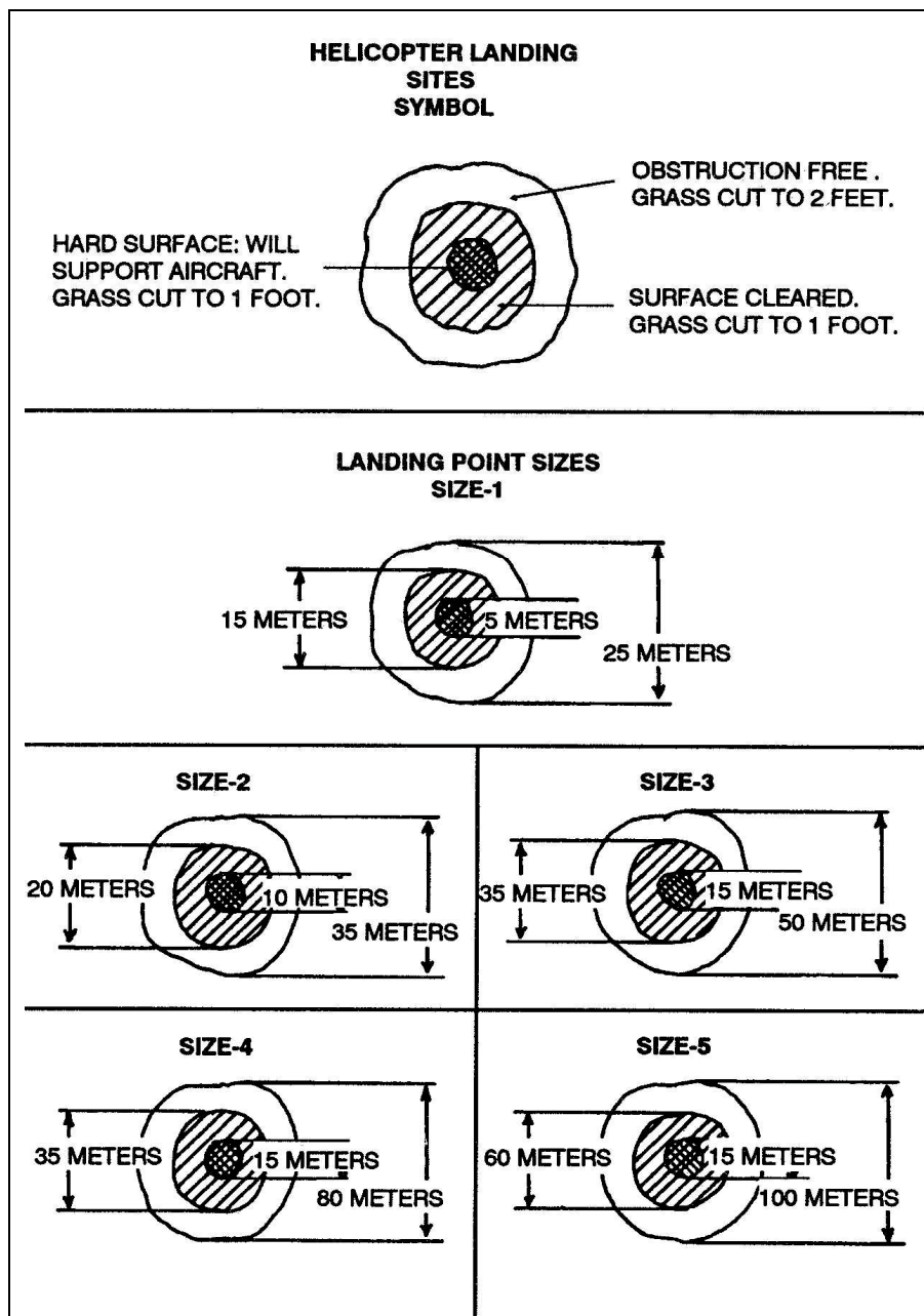
Figure 4-3. Landing points.
