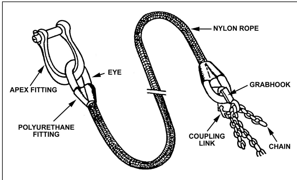
Figure 5-9. 25,000-pound capacity sling set.
