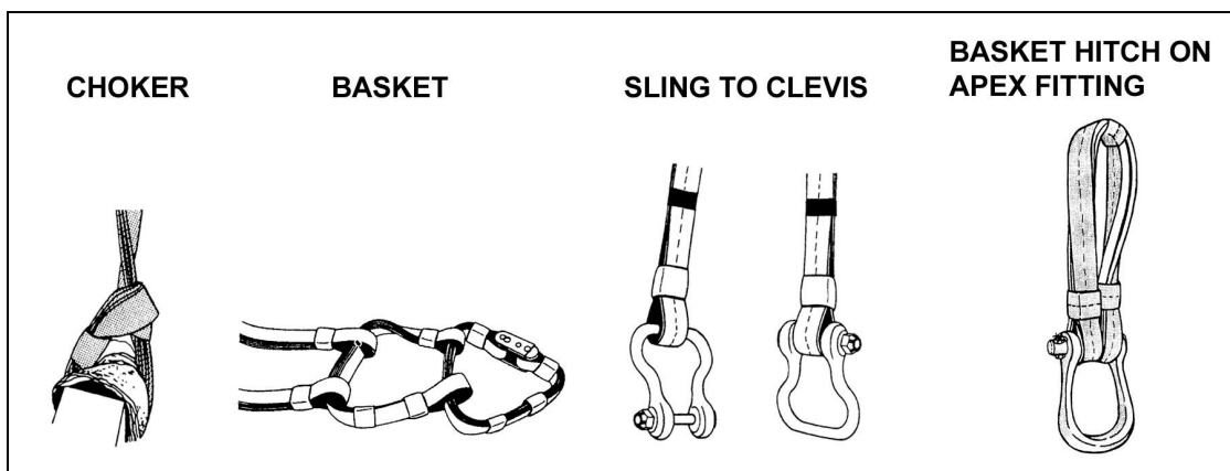
Figure 5-1. Hitches.
