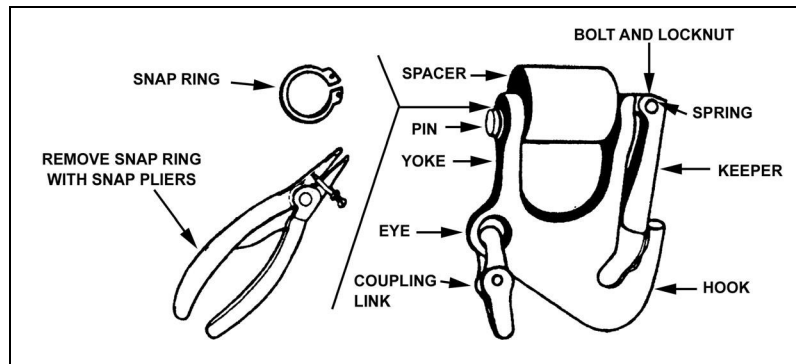
Figure 5-12. Grabhook.
