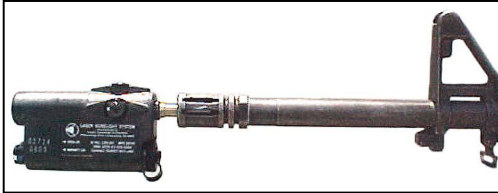
Figure 8-4. Borelight in the HALF TURN position.
