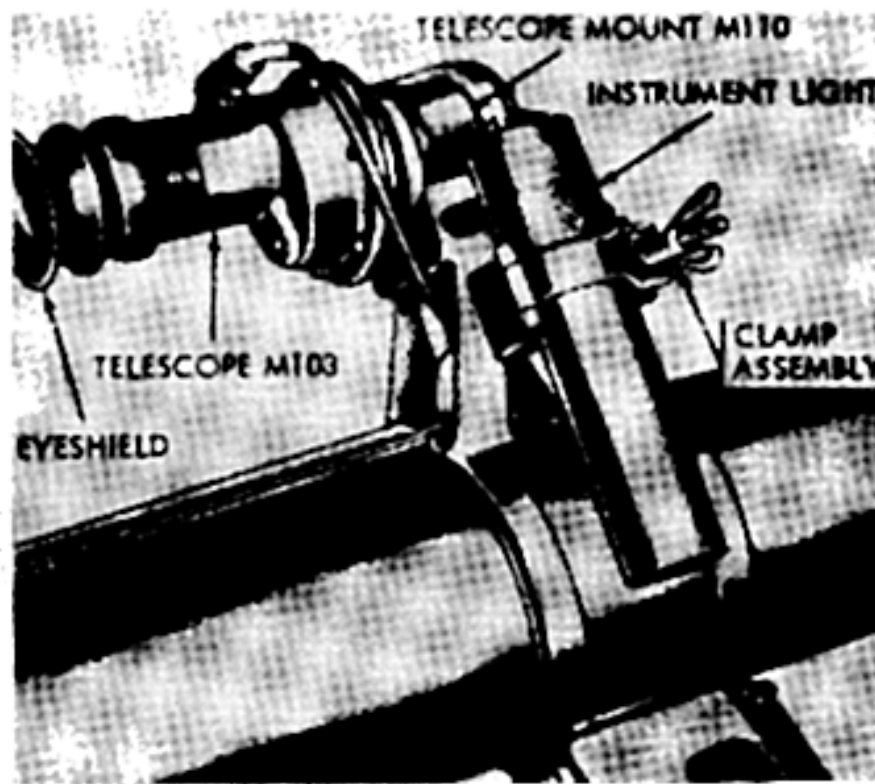
Figure 5. Instrument Light, T25.
