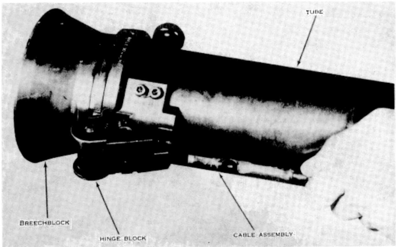
Figure 9. Removing and installing the cable assembly.
