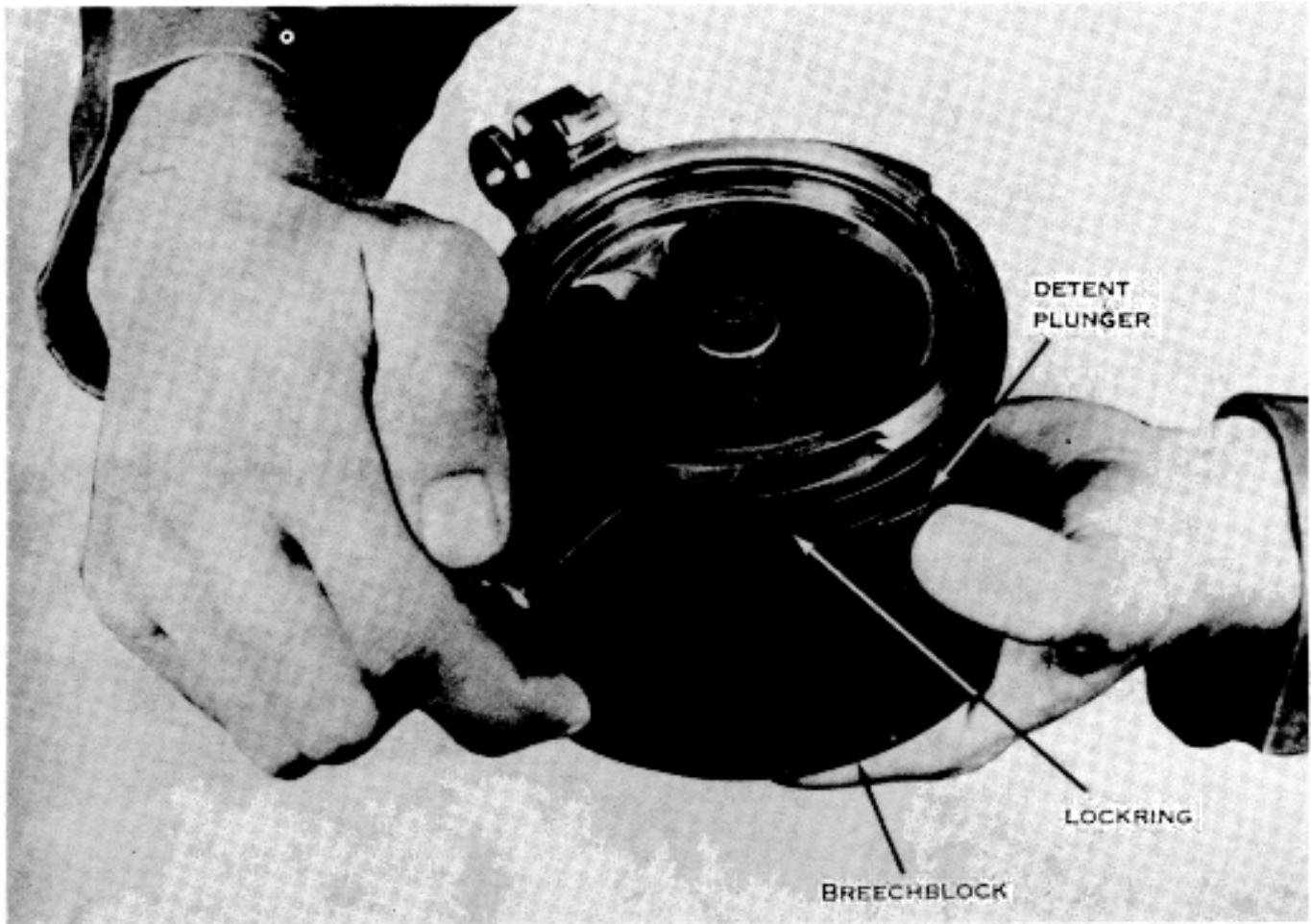
Figure 11. Removing the lockring.
