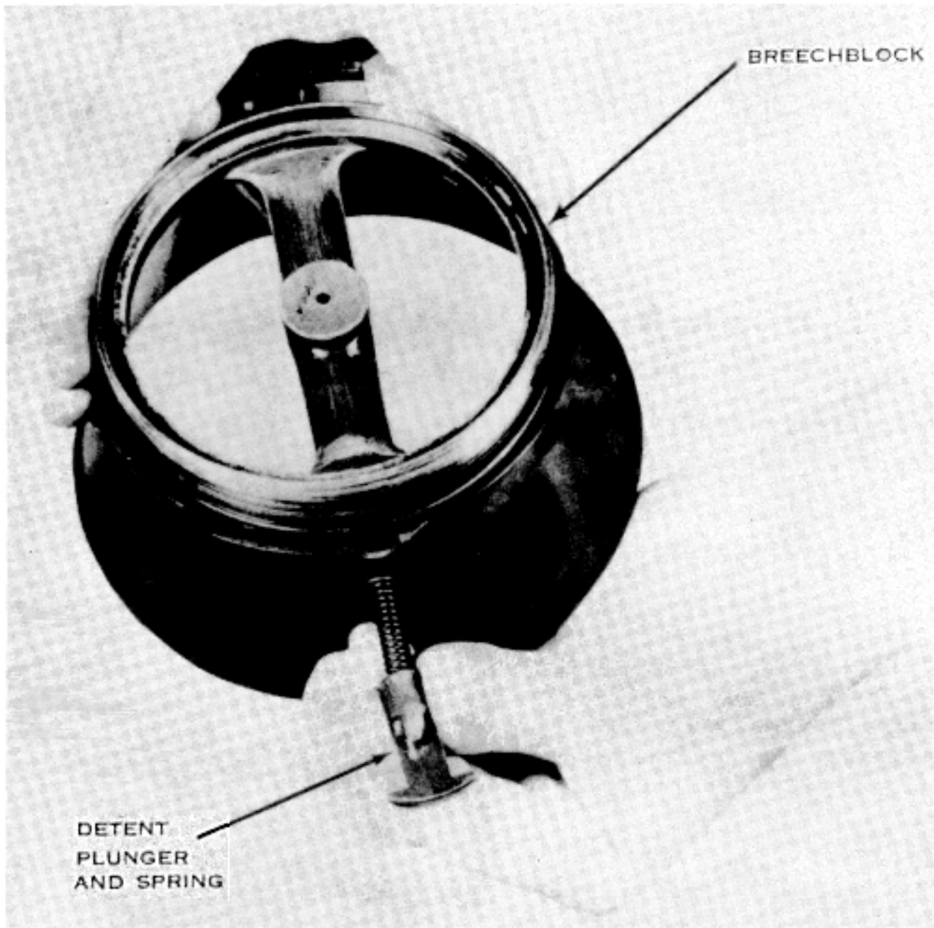
Figure 13. Removing the detent plunger and spring.
