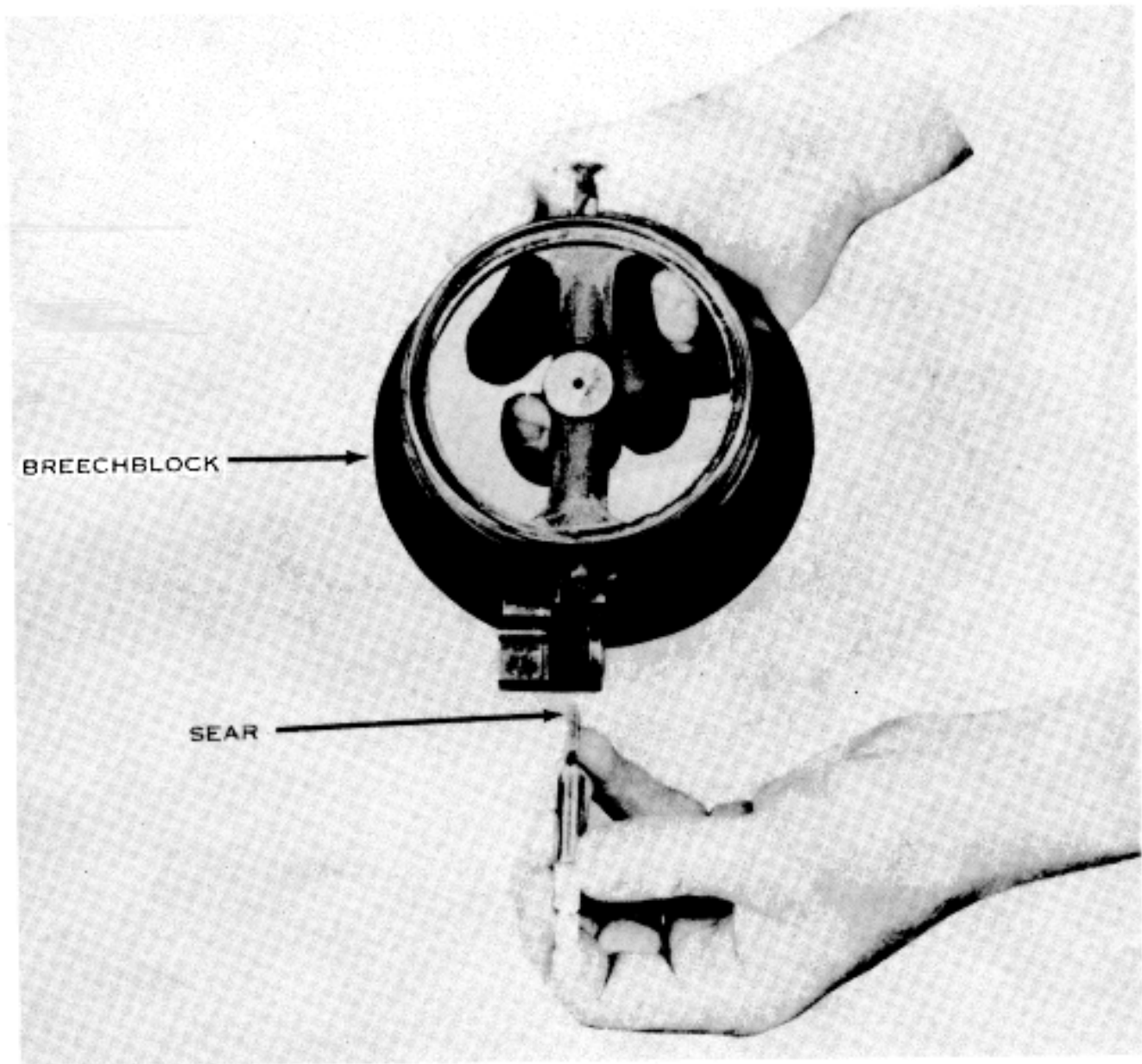
Figure 12. Removing the sear.
